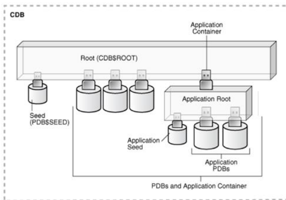
Figure 1-1 Multi-Tenant Architecture
