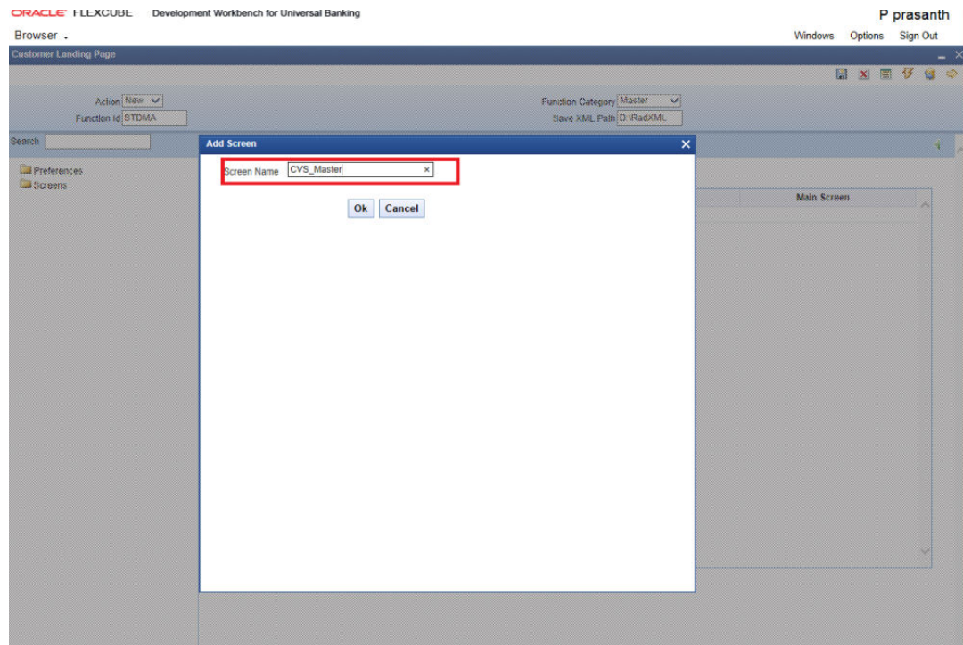
Figure 2-3 Add Screen
