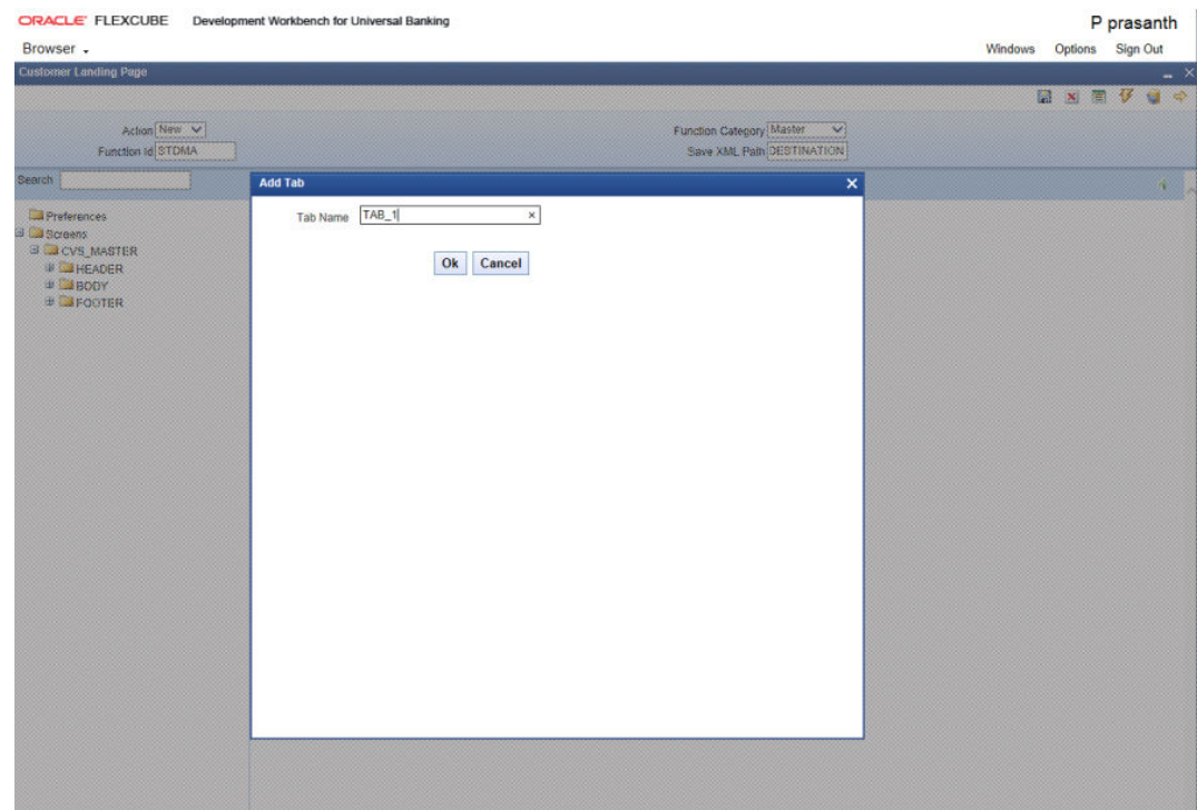
Figure 2-6 Add Tab
