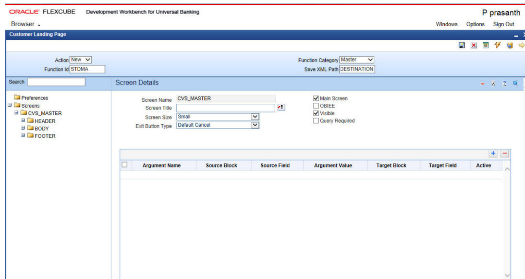
Figure 2-4 Screen Details
