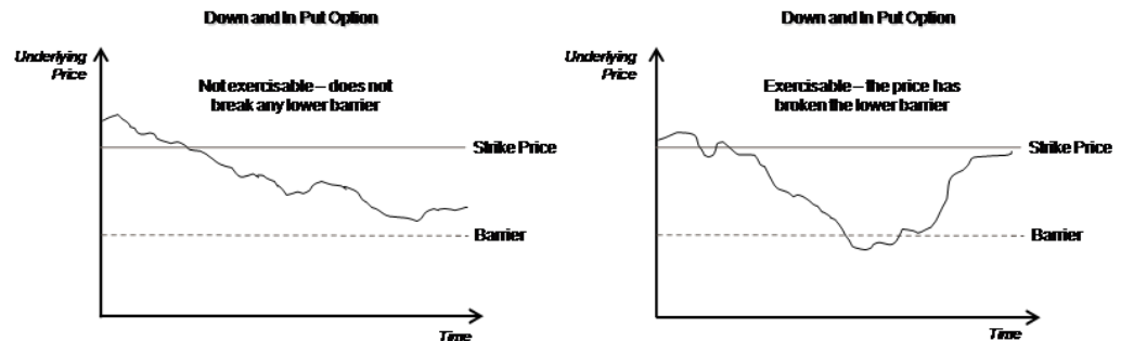
Figure 3-7 Down and In put option
