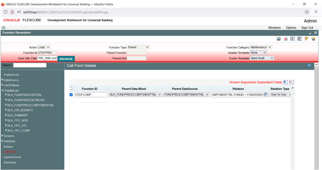
Figure 2-31 Call Form Details
