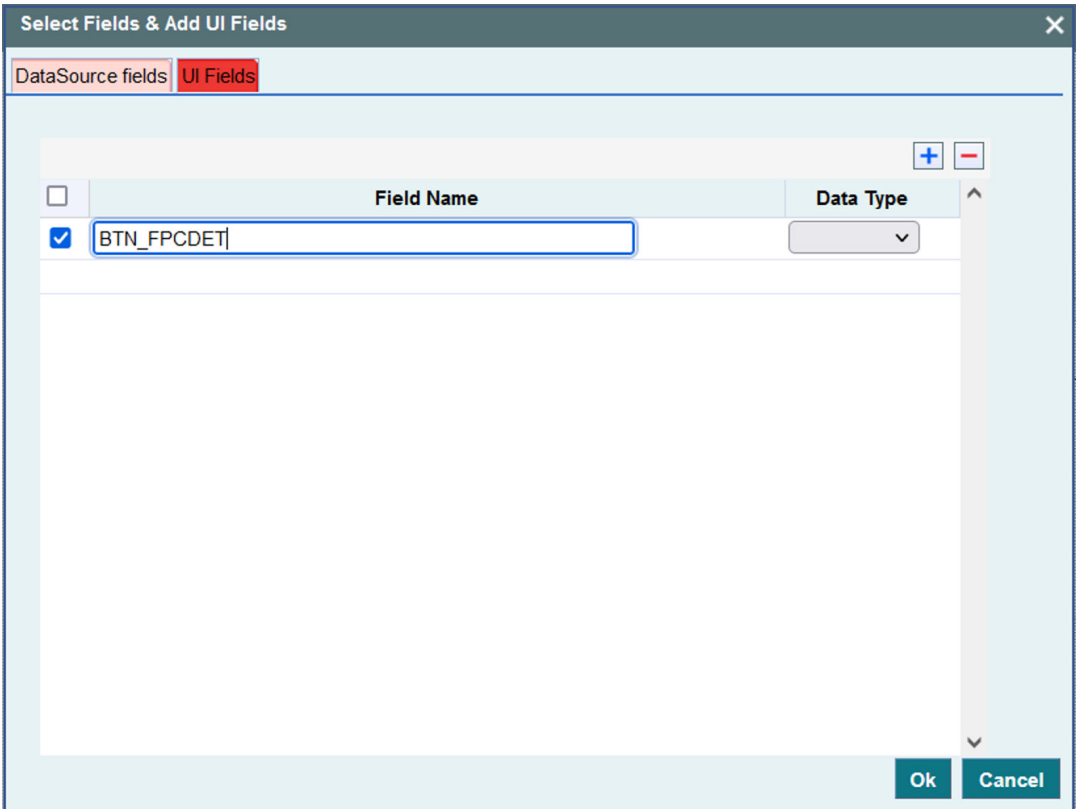
Figure 2-30 Defining Button field
