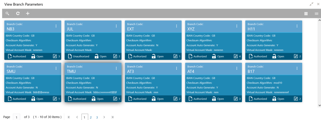
Figure 5-2 View Branch Parameters
