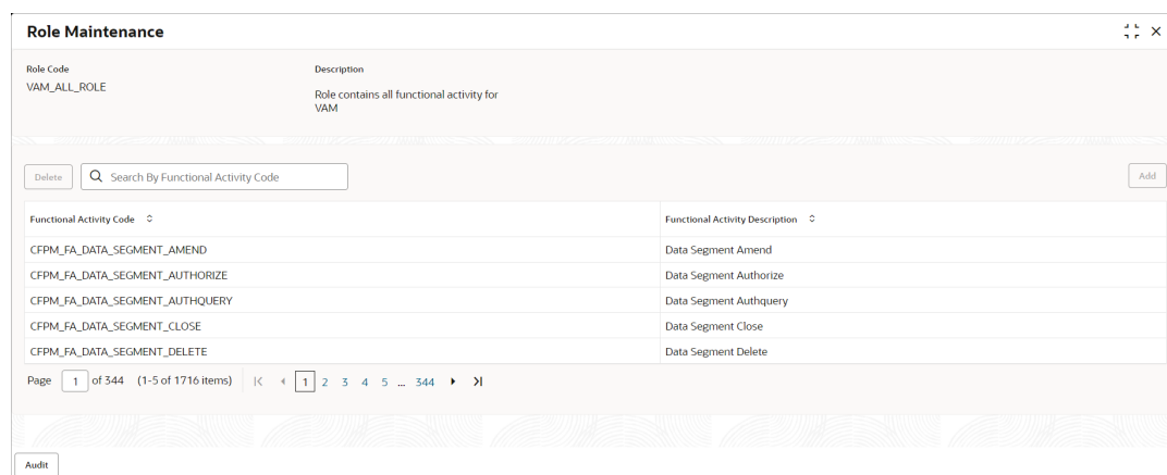
Figure 4-3 Role Maintenance
