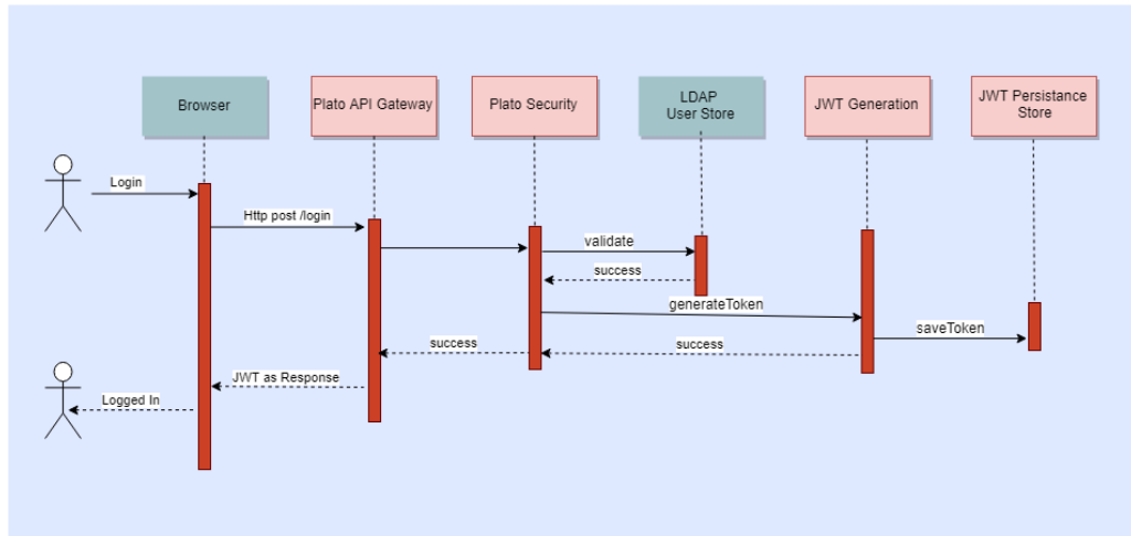
Figure 1-1 LDAP Authentication
