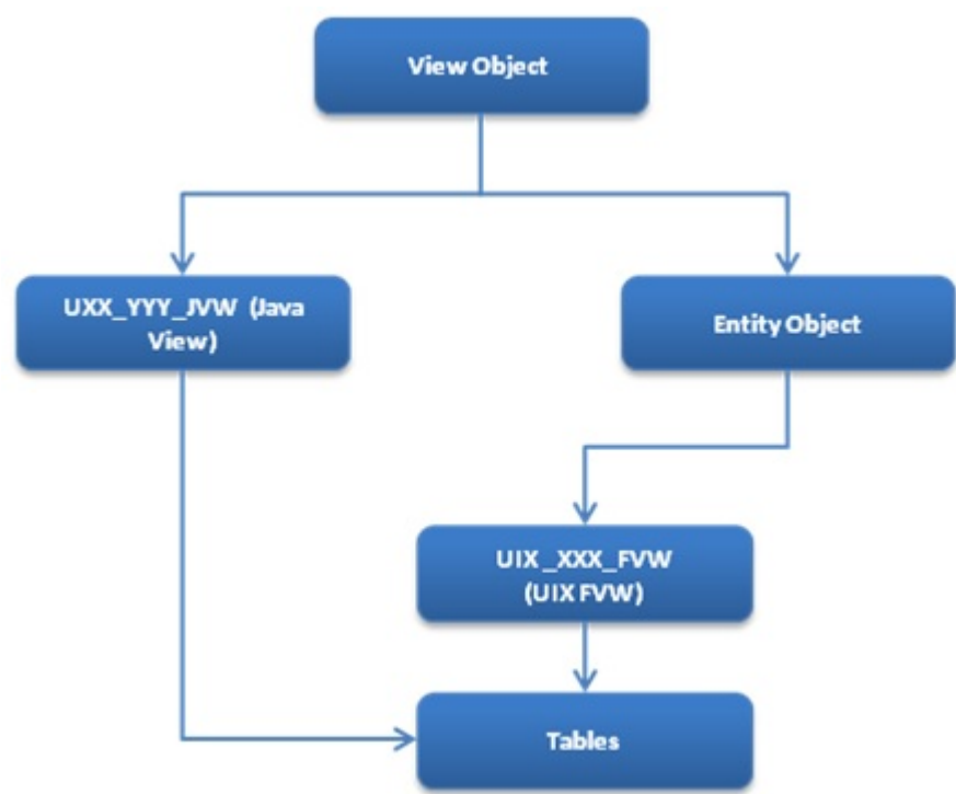
Figure 4-3 Database Schema
