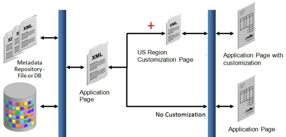
Figure 1-1 Customization Layers 1
