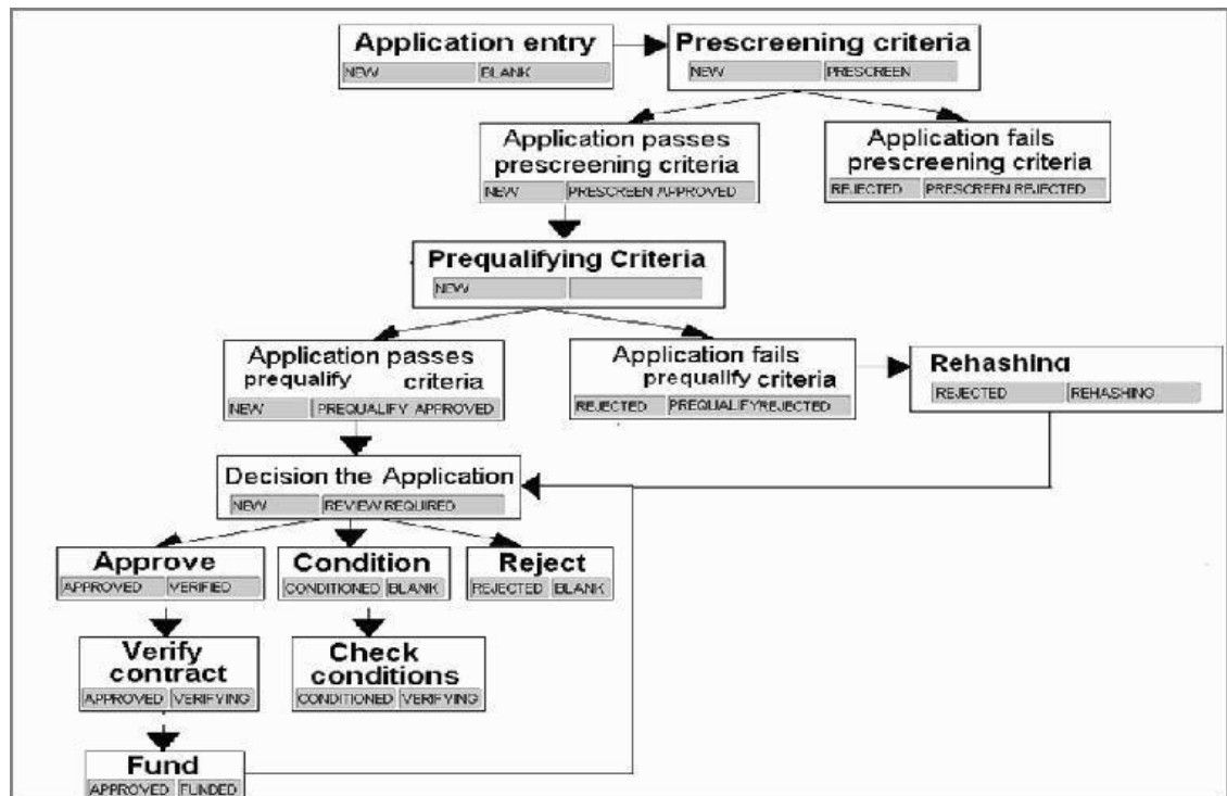
Figure 4-11 Application Entry - Flowchart 2
