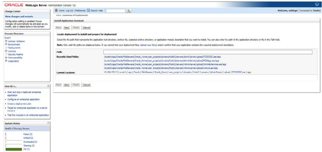
Figure 1-4 Deployments_Install
