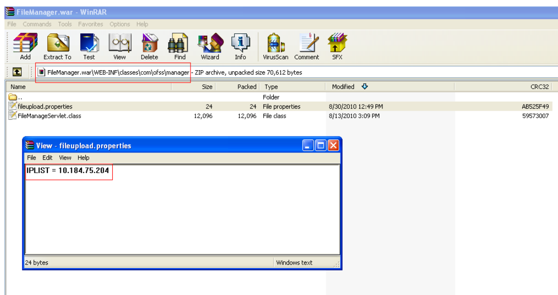
Figure 6-1 fileupload.properties
