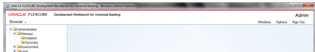
Figure 4-1 User Options
