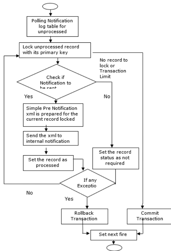
Figure 1-14 Flow Chart for Notification Flow in Scheduler
