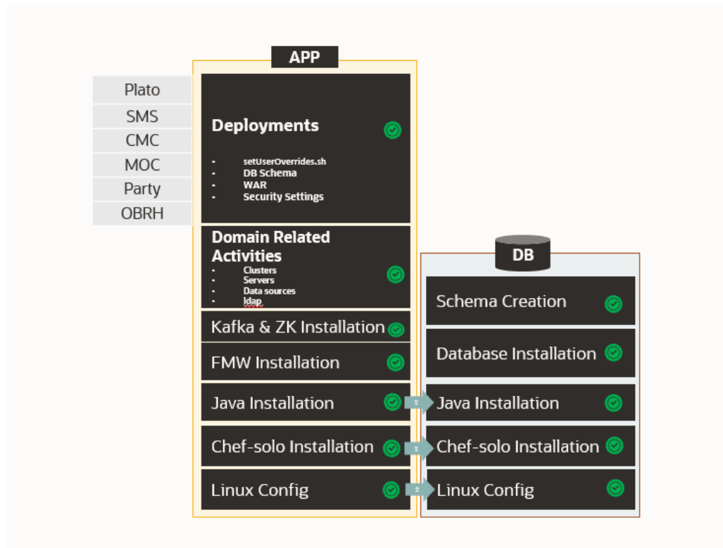
Figure 1-2 Oracle Banking Microservices Architecture Installation
