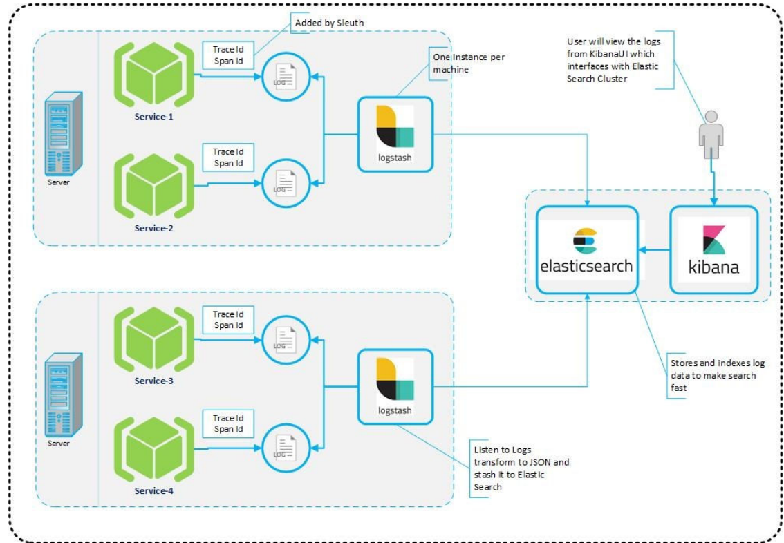
Figure 2-1 Architecture
