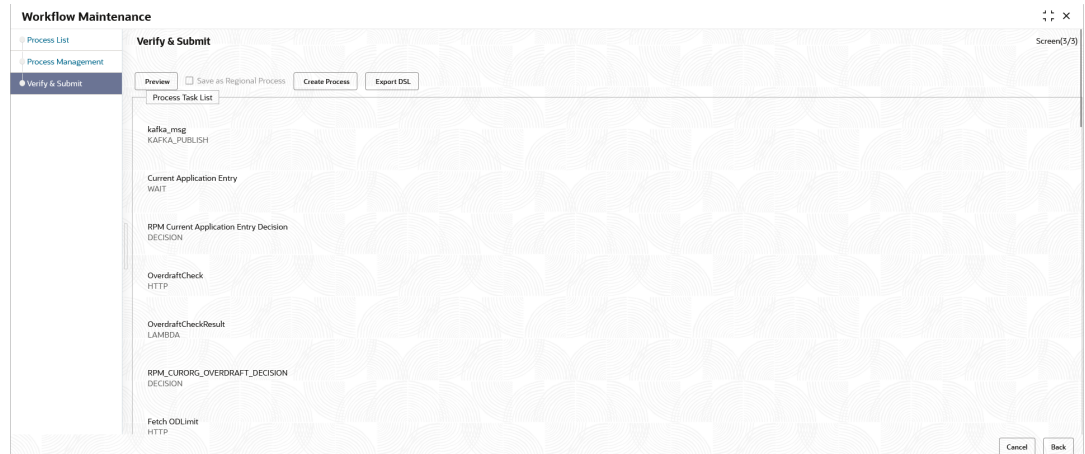
Figure 1-22 Verify & Submit
