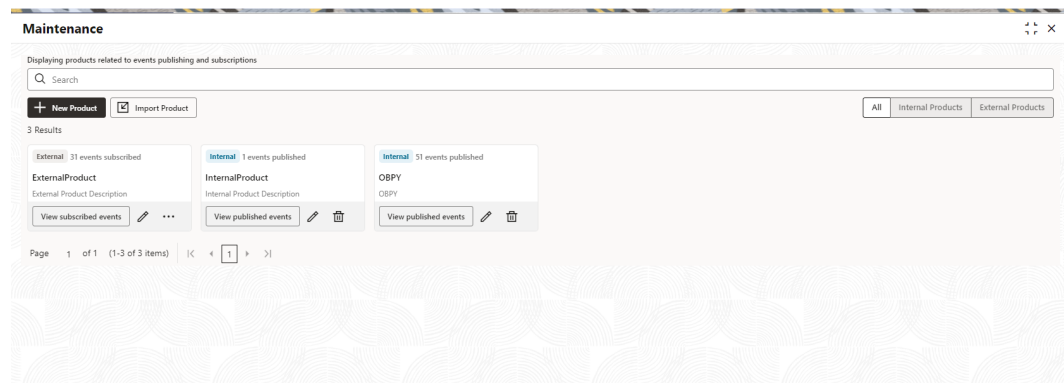
Figure 1-33 Event Maintenance
