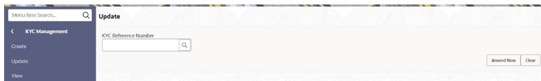
Figure 3-3 Update
