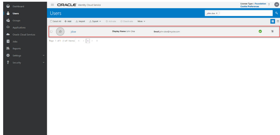
Figure 5-2 Users Window
