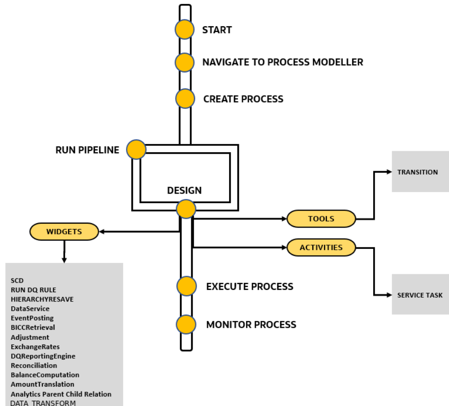
Figure 17-1 Process Pipeline Flow
