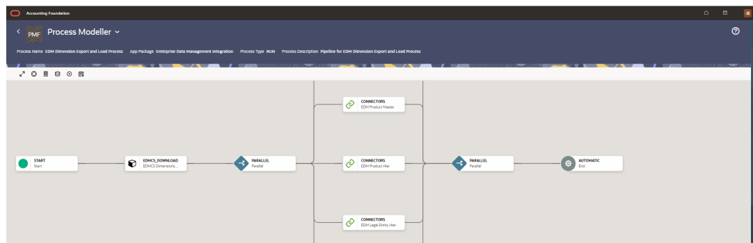
Figure 13-9 EDMCS Pipeline
