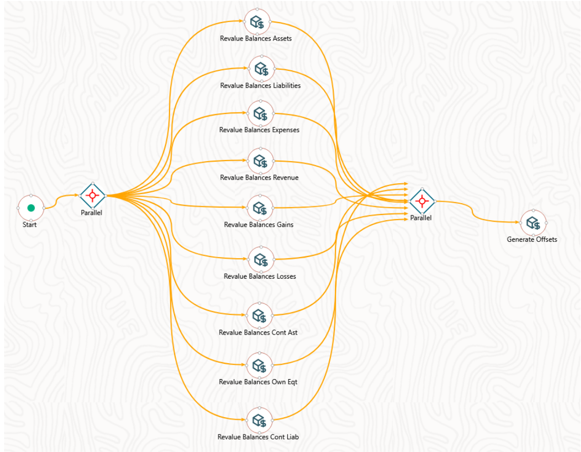
Figure 17-15 Executing Parallel Tasks flow
