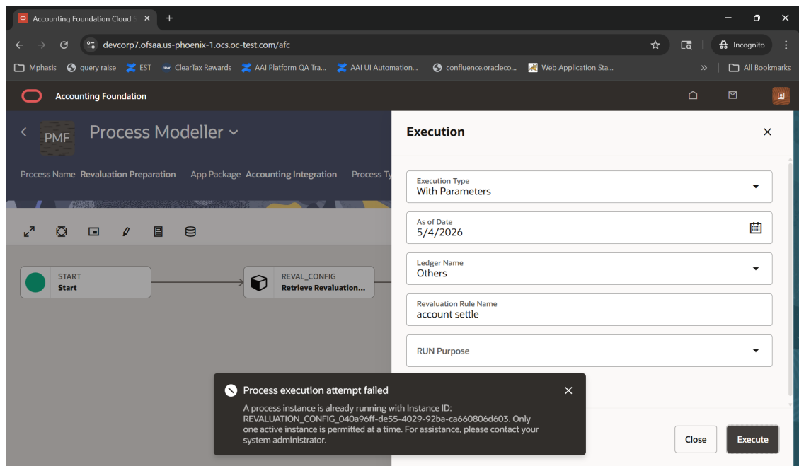
Figure 17-13 Re-execution Error of a Singleton Pipeline
