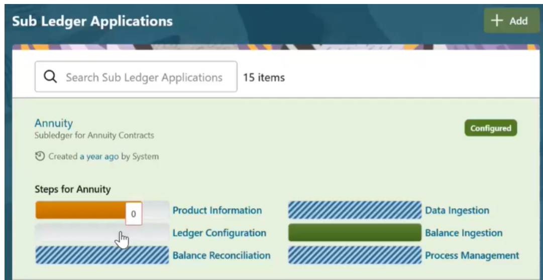
Figure 13-3 Subledger Configuration for Annuity_step 1
