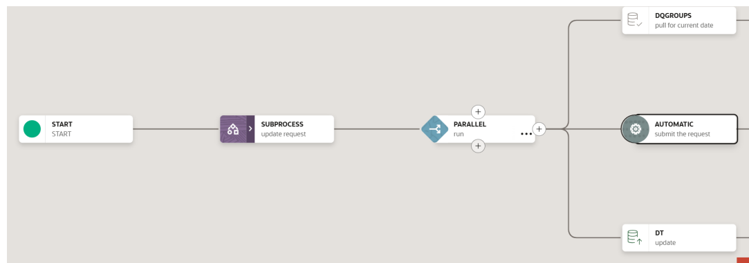
Figure 17-10 Create Sub run pipeline
