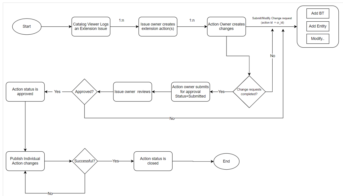
Figure 21-1 Approval Workflow for Issues and Actions
