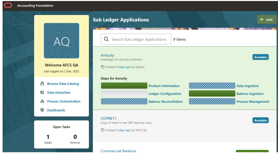
Figure 12-1 Subledger Application
