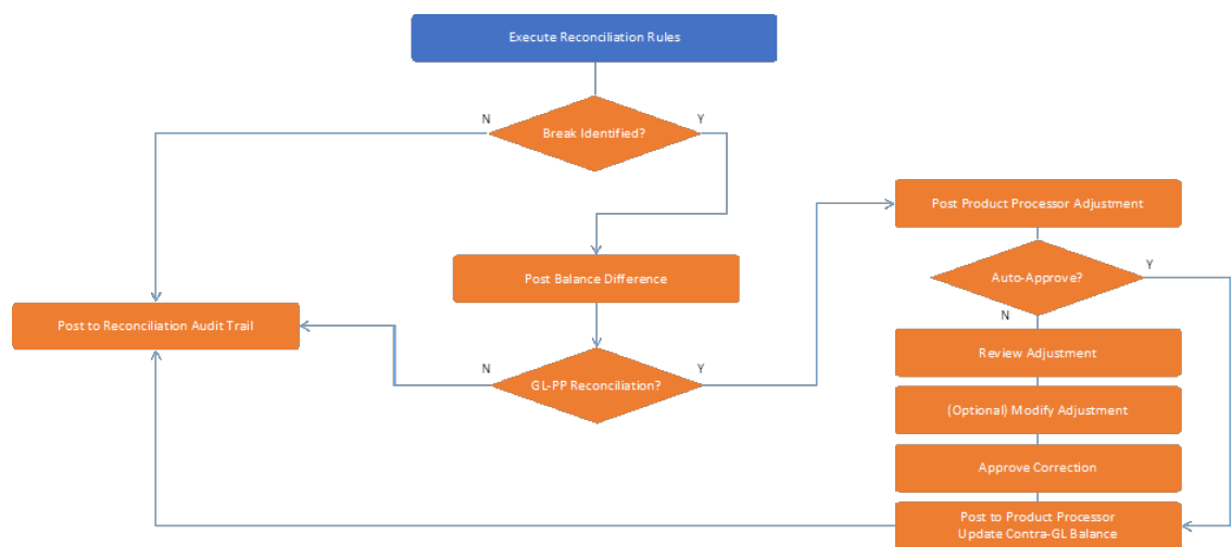
Figure 19-3 Balance Reconciliation Rule for General Ledger to Product Processor Workflow
