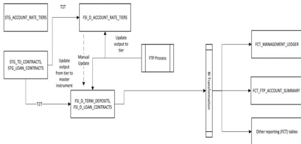
Figure 21-2 FTP Data Flow
