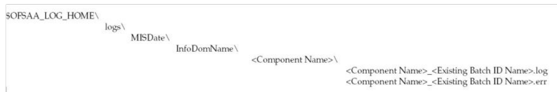
Figure 7-42 Folder Structure of Execution Logs
