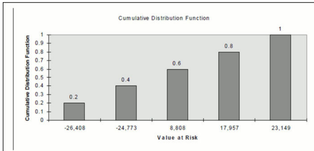
Figure 13-6 Cumulative Distribution Function
