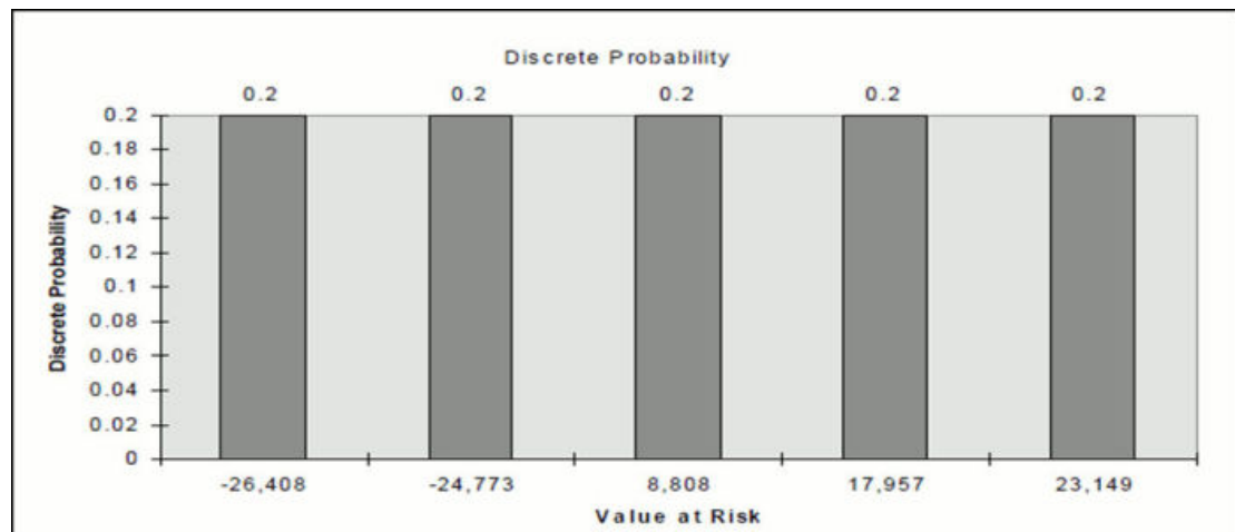
Figure 13-3 Graph of Discrete Probability
