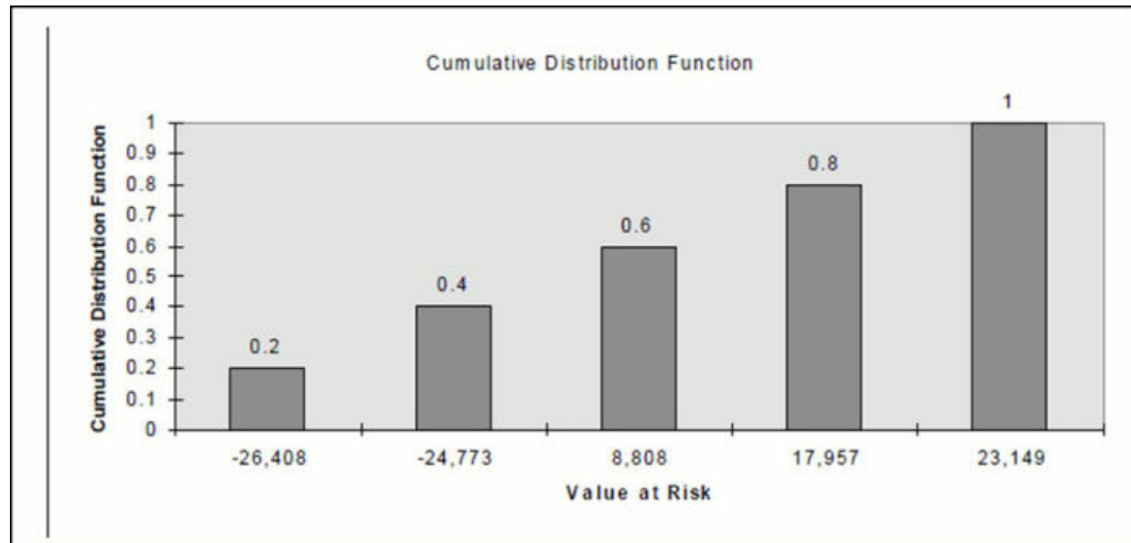
Figure 13-4 Graph of Cumulative Distribution Program
