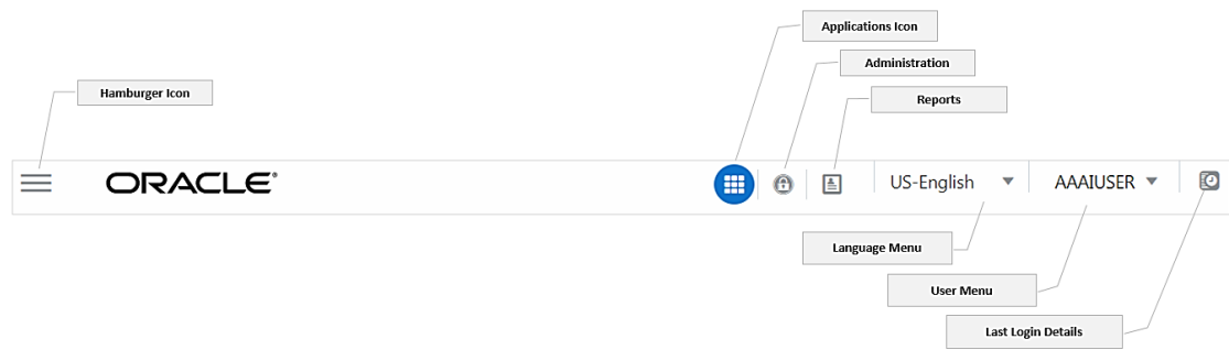
Figure 3-6 OFSSA Header
