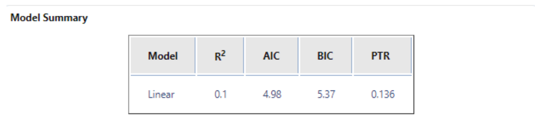
Figure 26-6 Model Summary
