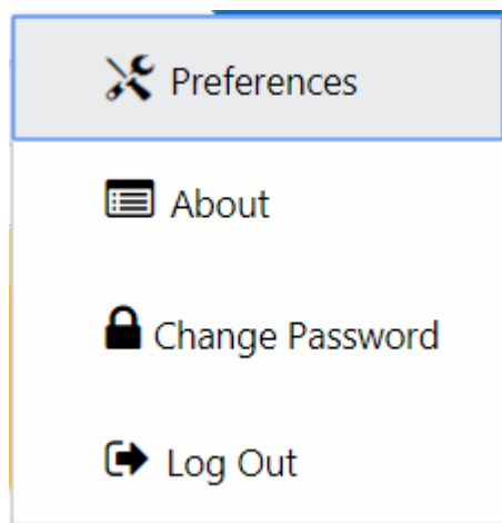
Figure 3-7 User Menu
