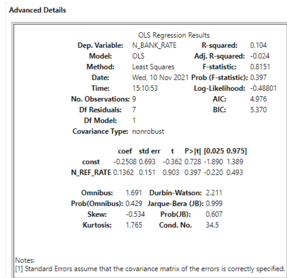
Figure 26-5 Advanced Details
