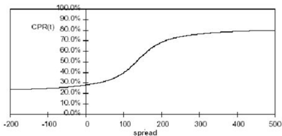
Figure 12-2 Prepayment Curve
