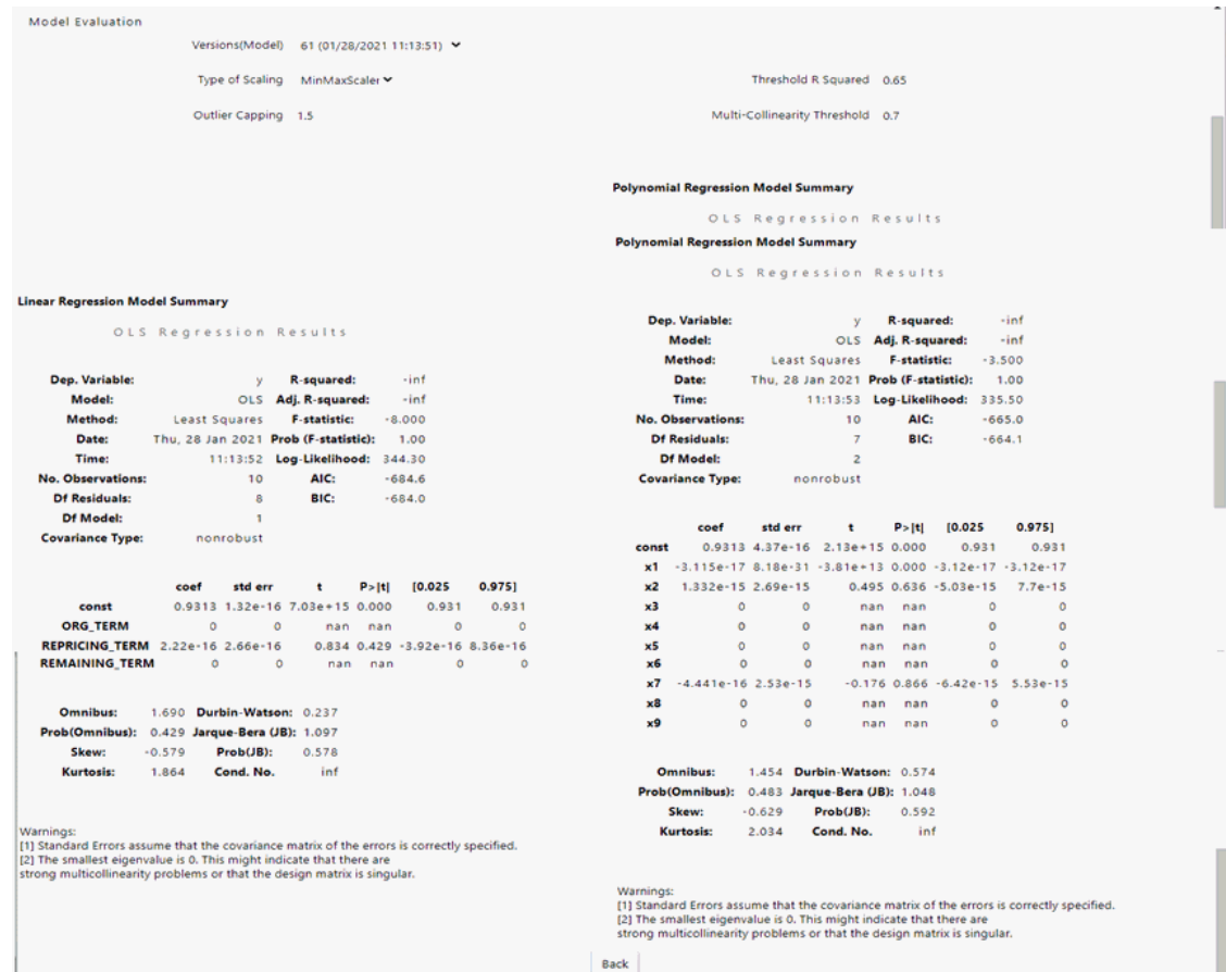
Figure 24-11 Advance Details
