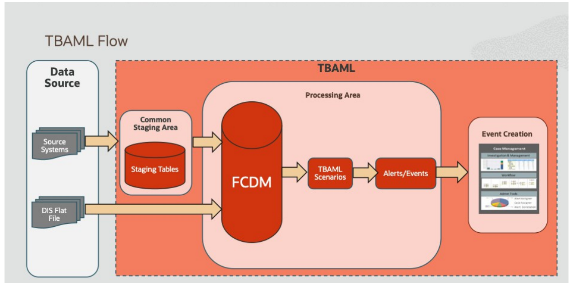
Figure 2-2 TBAML Architecture
