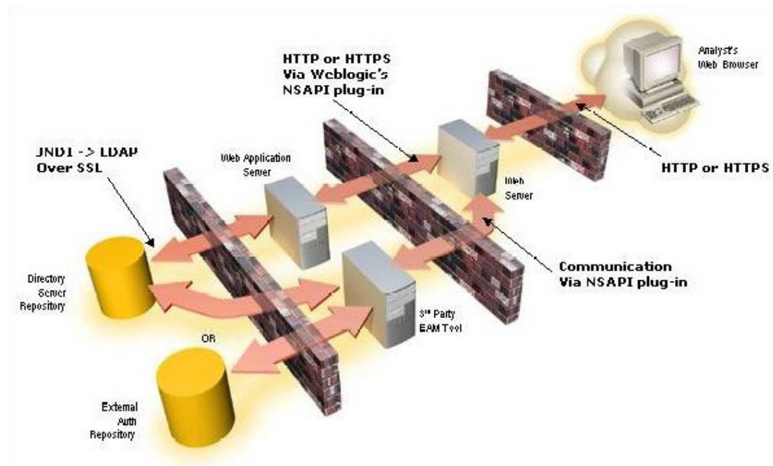
Figure 2-4 Security View
