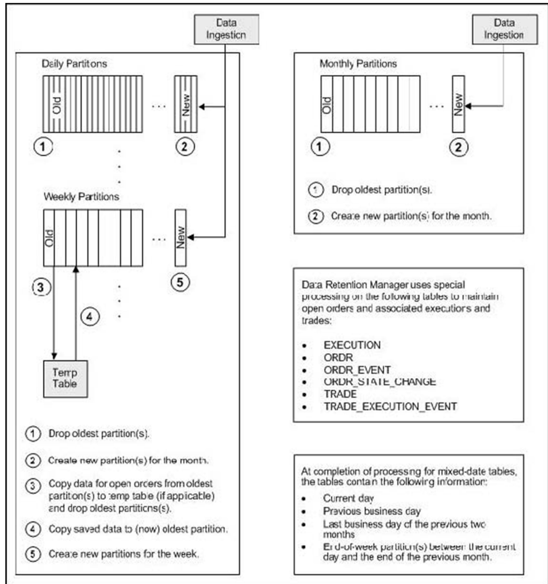
Figure 8-5 Database Partitioning Process
