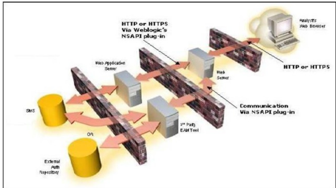
Figure 2-2 Oracle Financial Services/ Architecture—Security View
