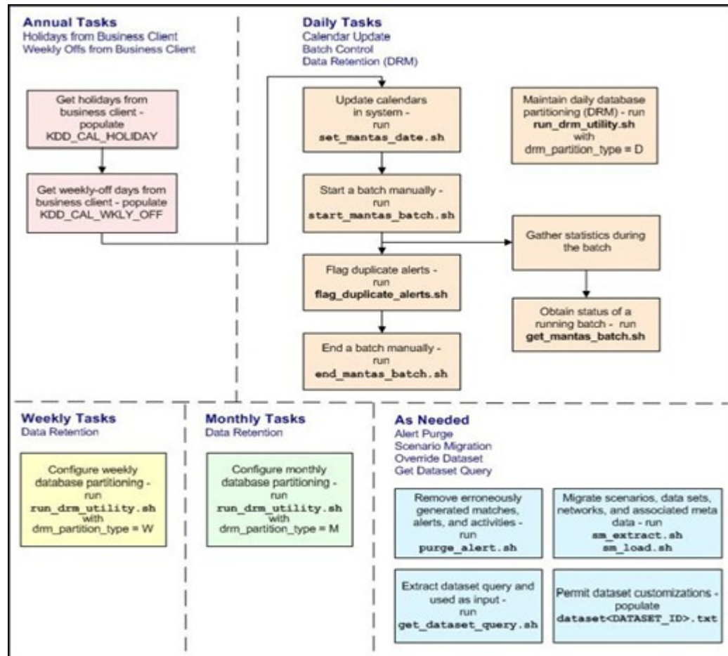
Figure 8-1 Managing Database Activities with Utilities
