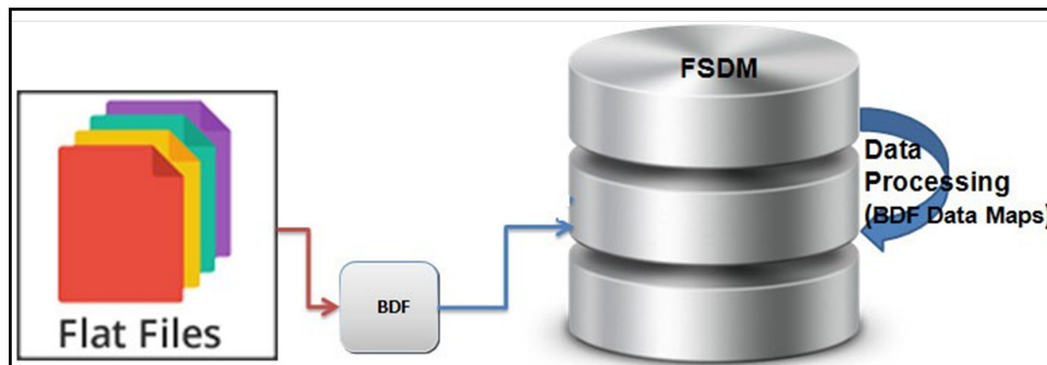
Figure 3-4 Data Loading Flow Using Flat File Interface
