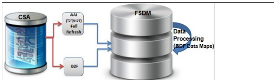
Figure 3-5 Data Loading For AML/Fraud/KYC/FATCA/CTR Applications
