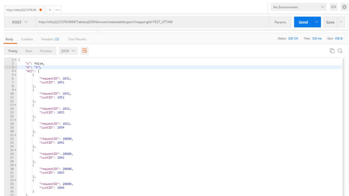
Figure 4-1 Sample JSON
