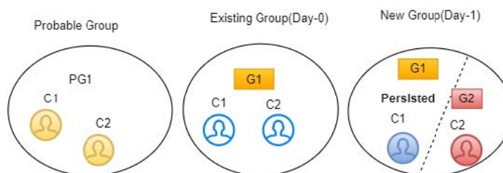
Figure 4-27 Split Action for Lowest Global ID
