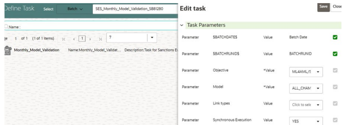
Figure 5-64 Edit Task for Monthly Model Validation
