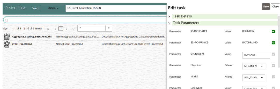
Figure 5-120 Edit Task for Aggregate_Scoring_Base_Features for Custom Scenario
