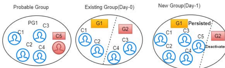
Figure 4-25 Merge and Add Action for Lowest Global ID
