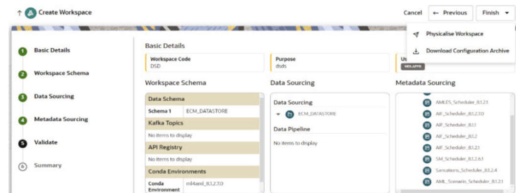
Figure A-20 Physicalise Workspace
