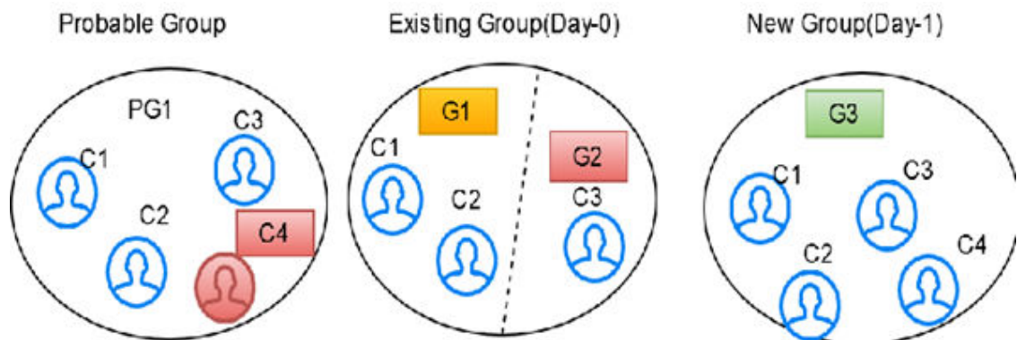
Figure 4-16 Merge and Add
