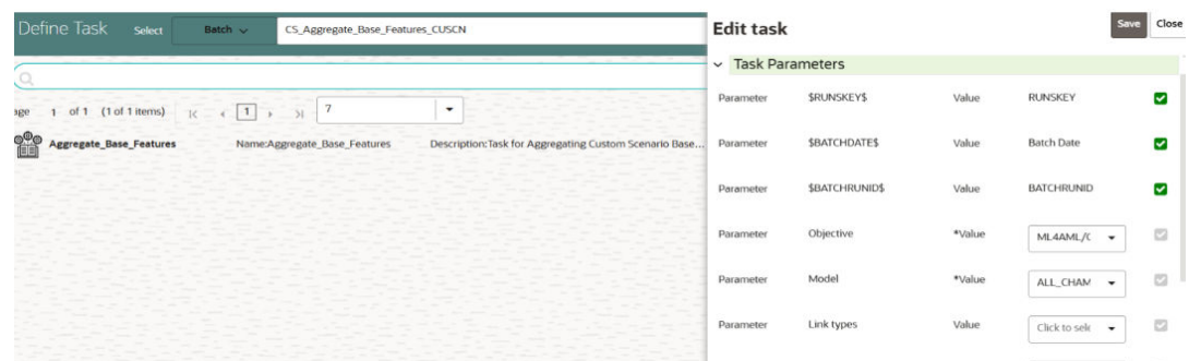
Figure 5-118 Edit Task for Aggregate Base Features
