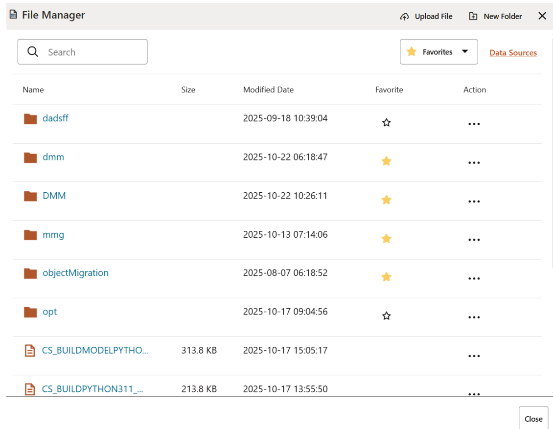
Figure 4-14 File Manager
