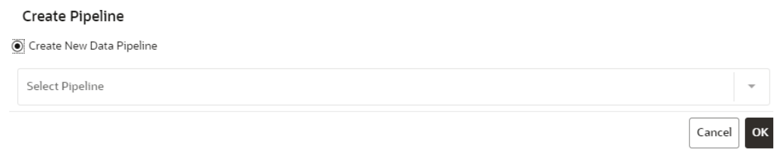
Figure 6-101 Create Pipeline
