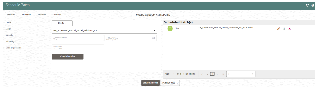
Figure 7-3 Scheduled Batches
