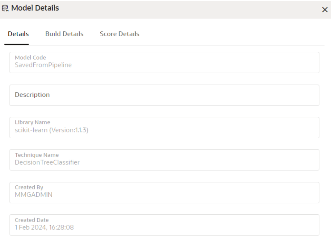
Figure 6-52 Model details
