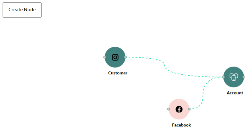
Figure 6-117 Graph page
