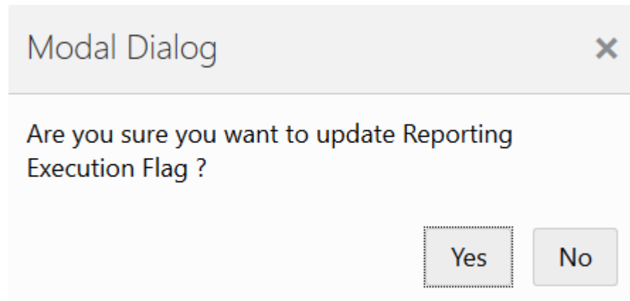
Figure 5-5 Modal Dialog
