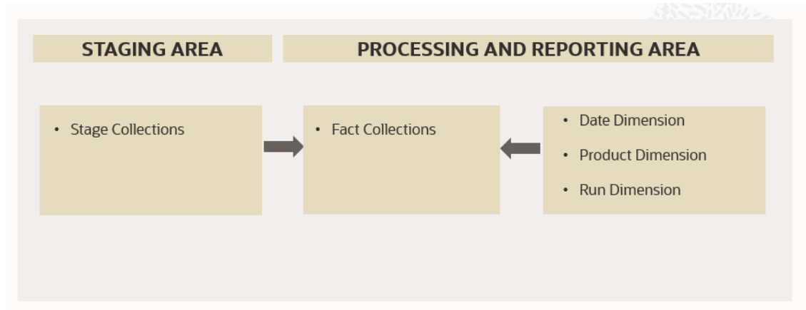
Figure 4-7 Collections Analysis
