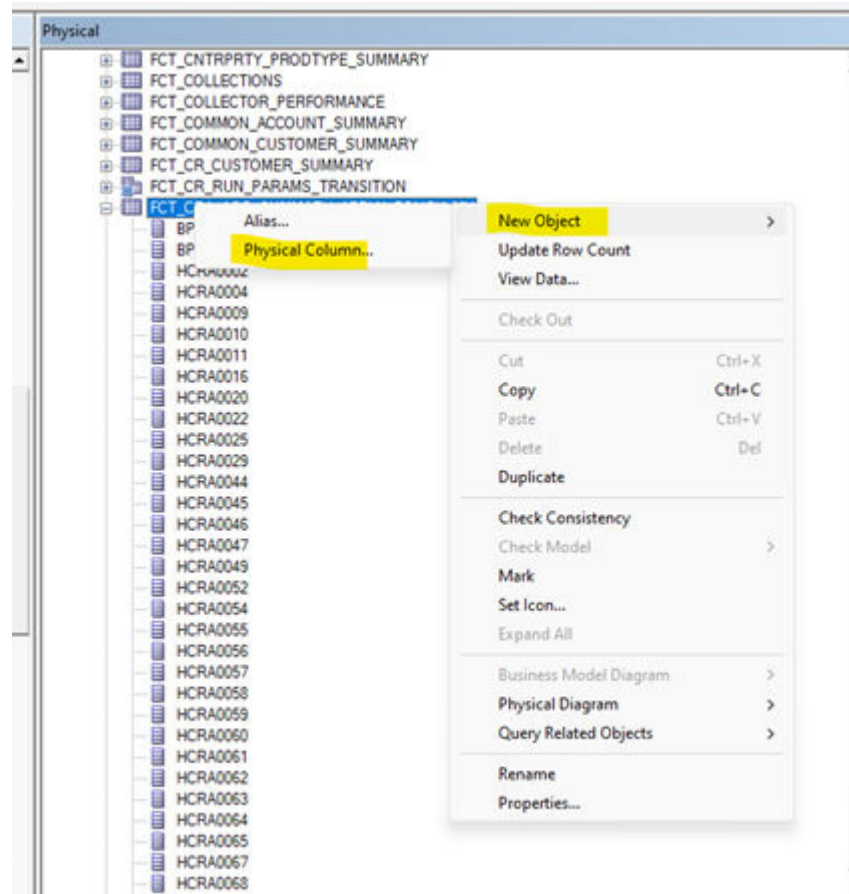
Figure 4-8 RPD screen
