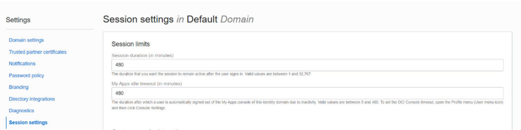
Figure 6-1 Session Settings
