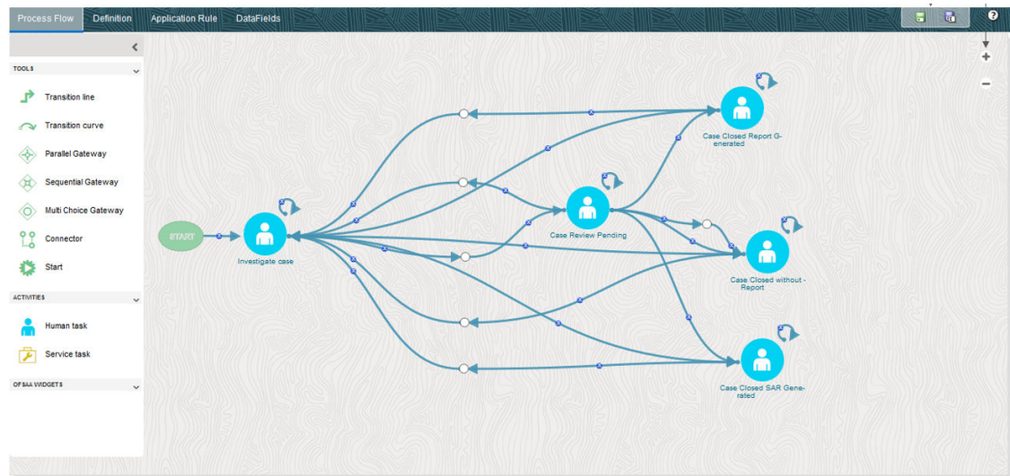
Figure 3-2 Drawing Canvas
