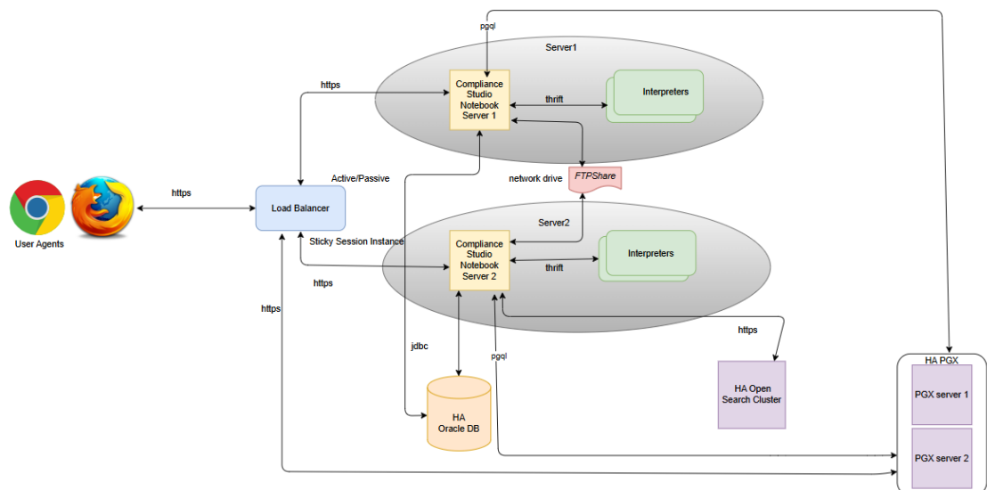
Figure 2-1 High Availability Architecture
