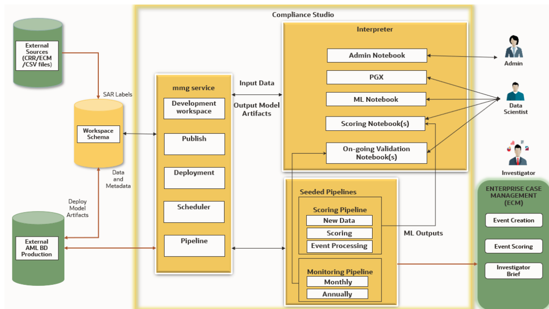
Figure 1-7 ML4AML
