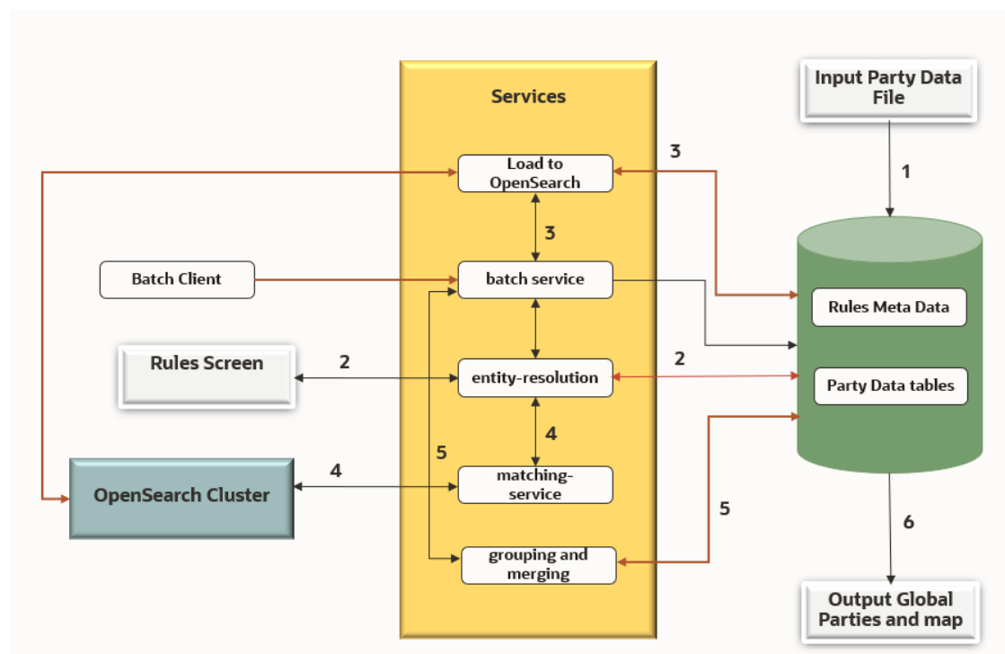
Figure 1-8 Entity Resolution
