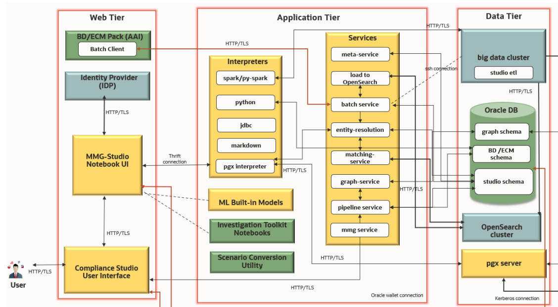
Figure 1-9 Investigation Toolkit
