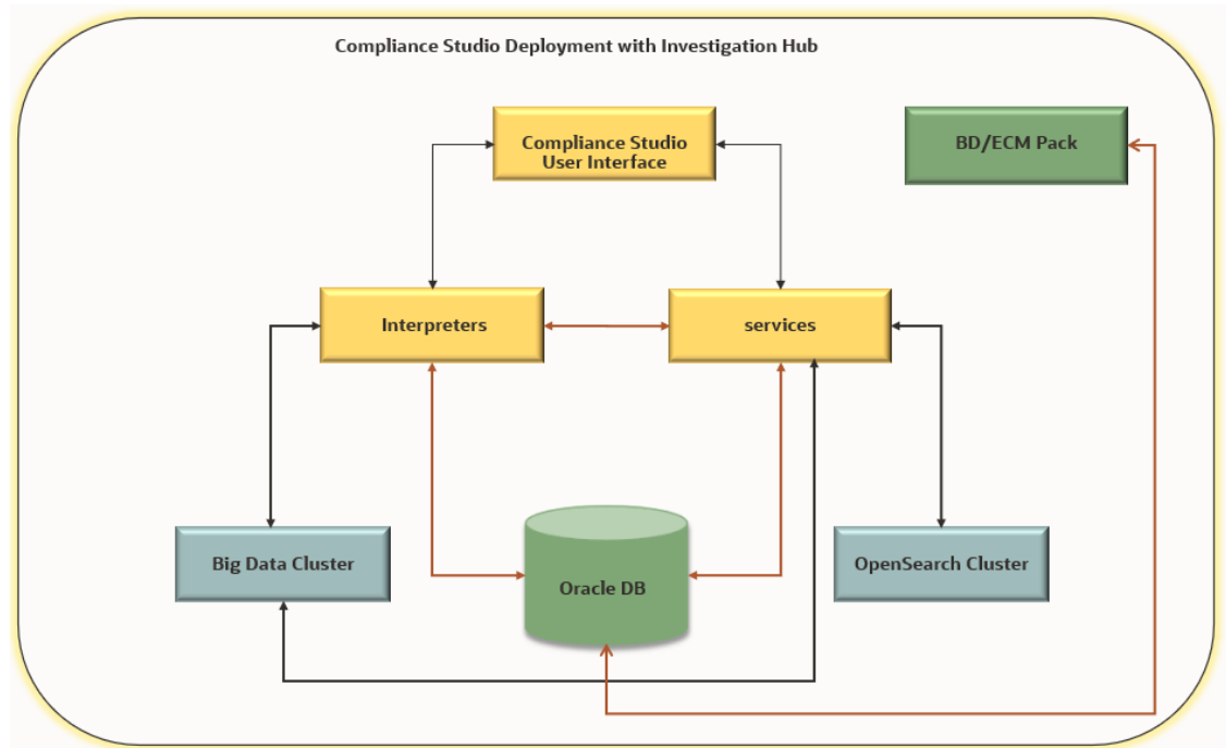
Figure 1-3 Simplify Architecture
