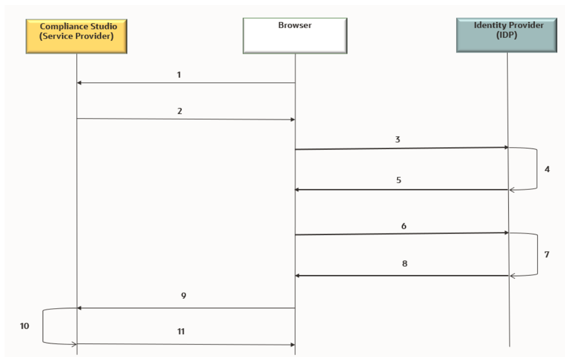
Figure 1-4 SAML Authentication Process
