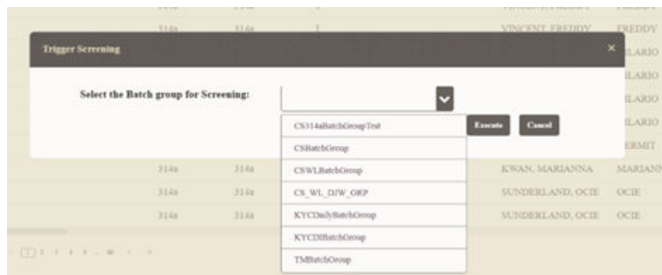
Figure 1-1 Trigger screening
