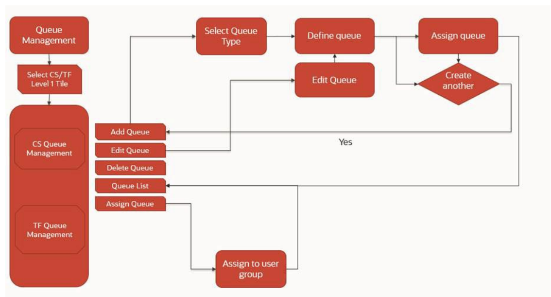
Figure 2-1 Queue Management Workflow
