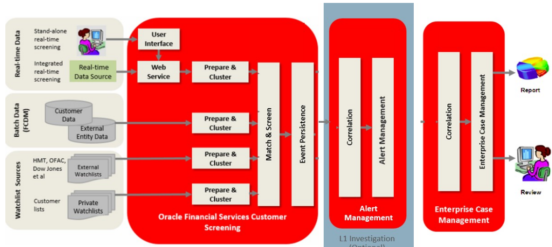
Figure 1-1 Customer Screening Architecture
