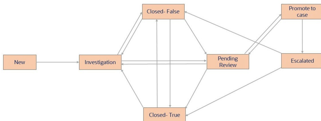
Figure 3-29 Promoting to Case PMF Work Flow
