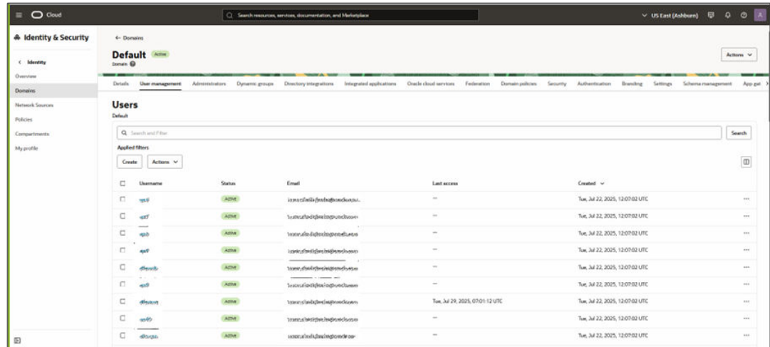
Figure 6-5 Users Mapped
