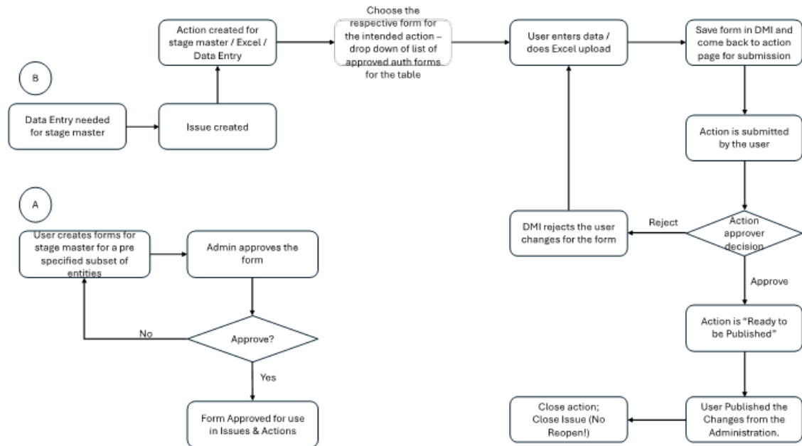
Figure 7-1 DMI Process Flowchart
