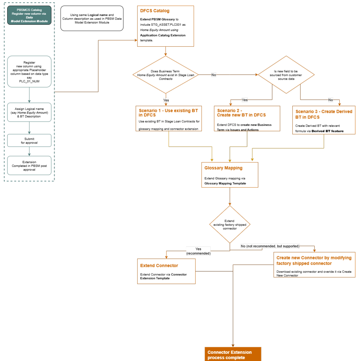
Figure 7-6 DFCS ADS Connectors
