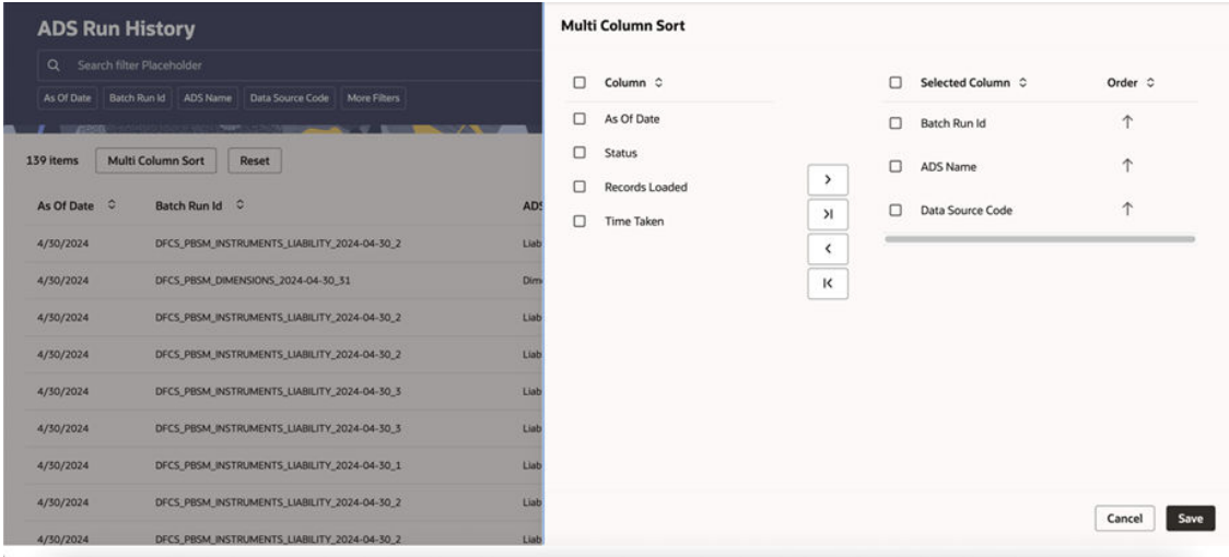
Figure 7-11 Multi Column Sort
