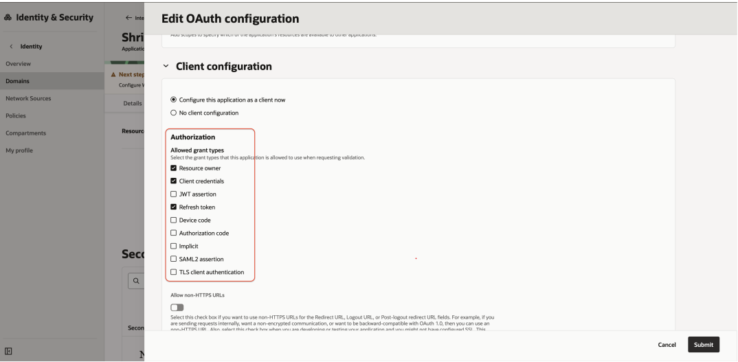
Figure 7-3 Client OAuth window
