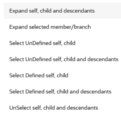
Figure 5-151 Member Tree
