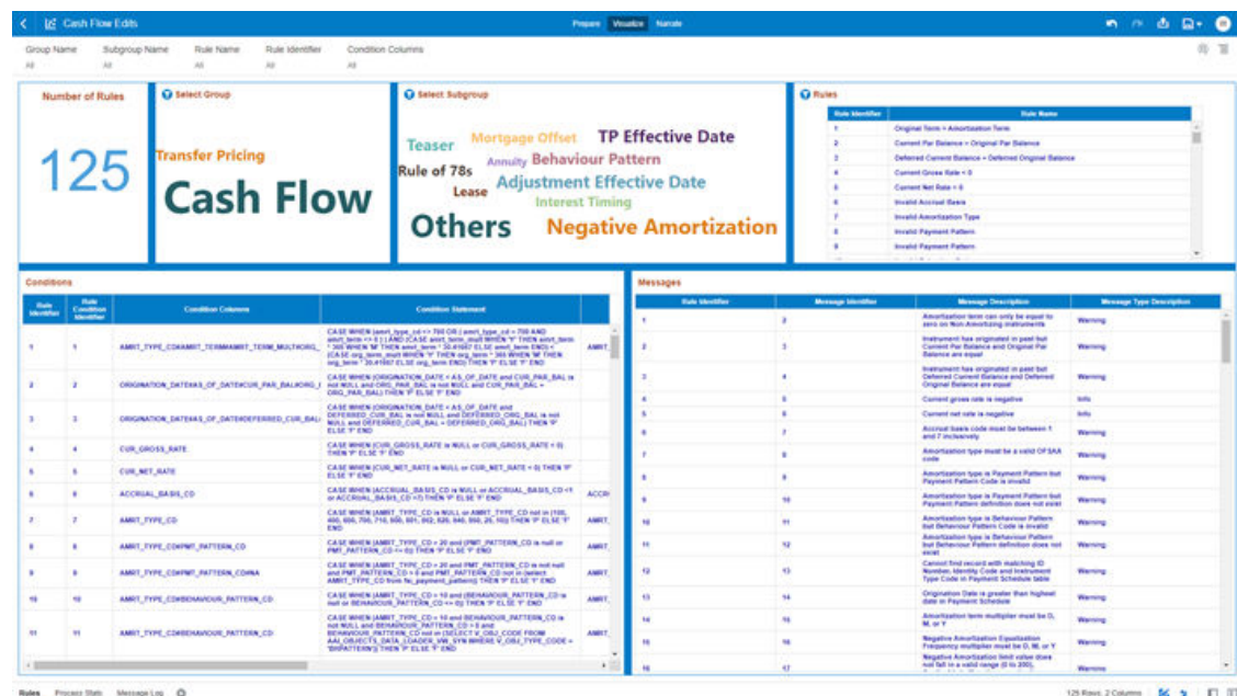
Figure 7-137 “Rules” Report
