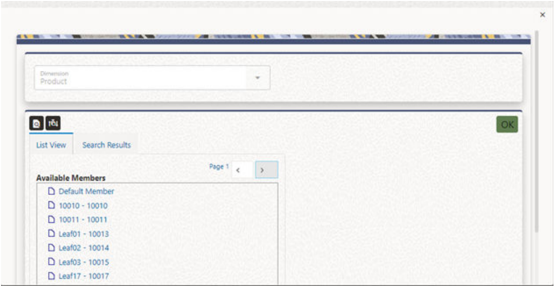
Figure 5-176 Hierarchy screen
