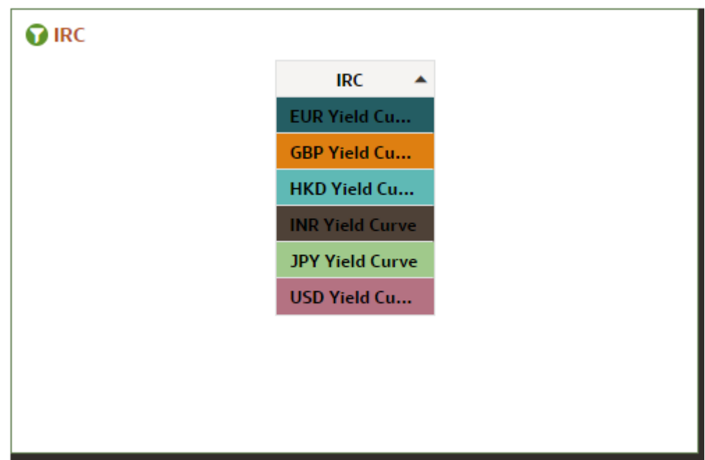
Figure 7-80 IRC Canvas
