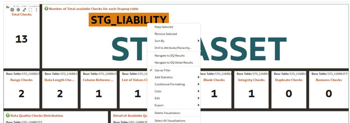
Figure 7-94 Data Action
