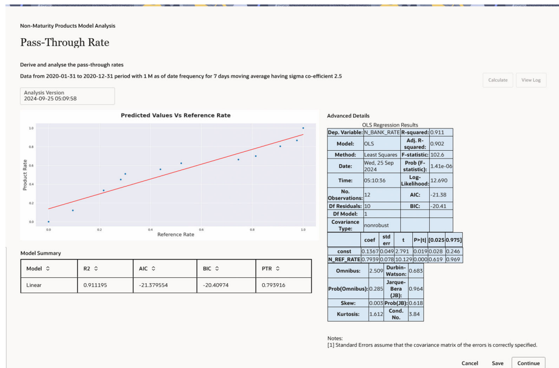
Figure 5-144 Pass-Through Rate
