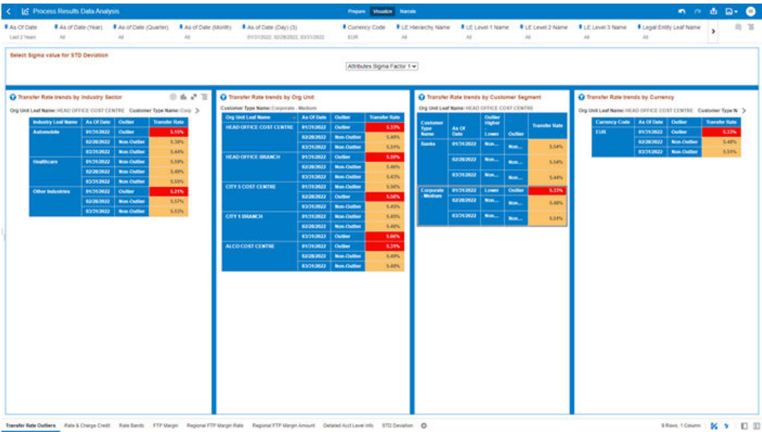
Figure 7-126 Outliers Selection
