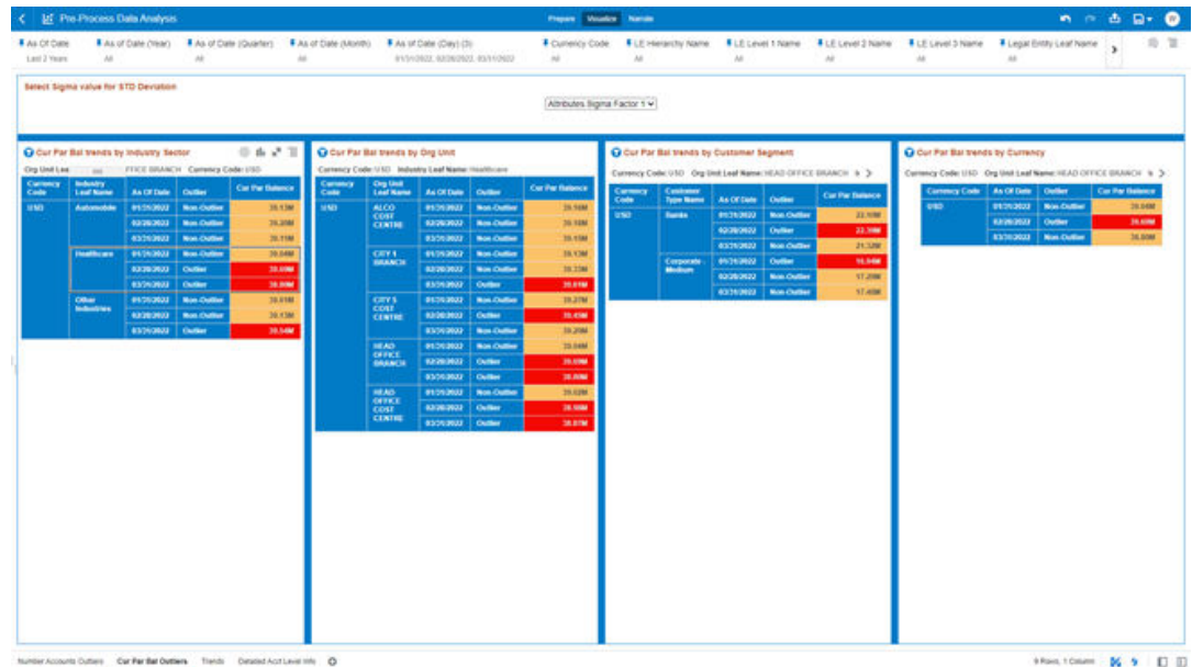
Figure 7-121 Outliers Selection
