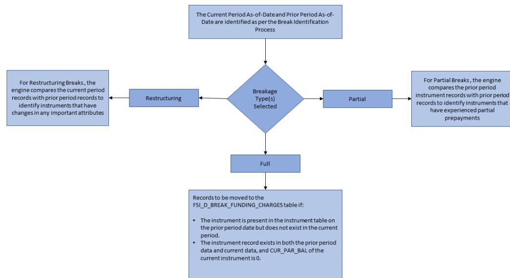
Figure 5-157 Break Identification Process Flow
