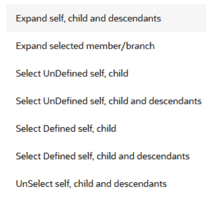
Figure 5-140 Member Tree
