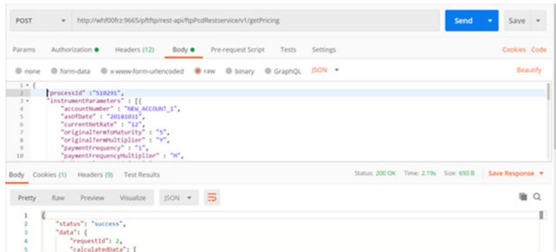
Figure L-4 Web API Testing Tool (example Postman)
