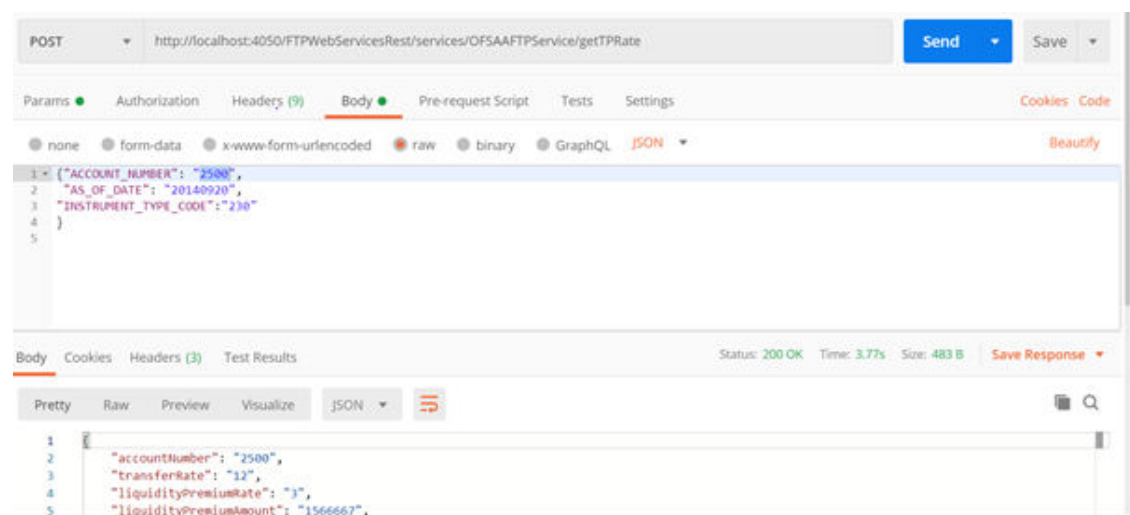
Figure L-2 Web API Testing Tool
