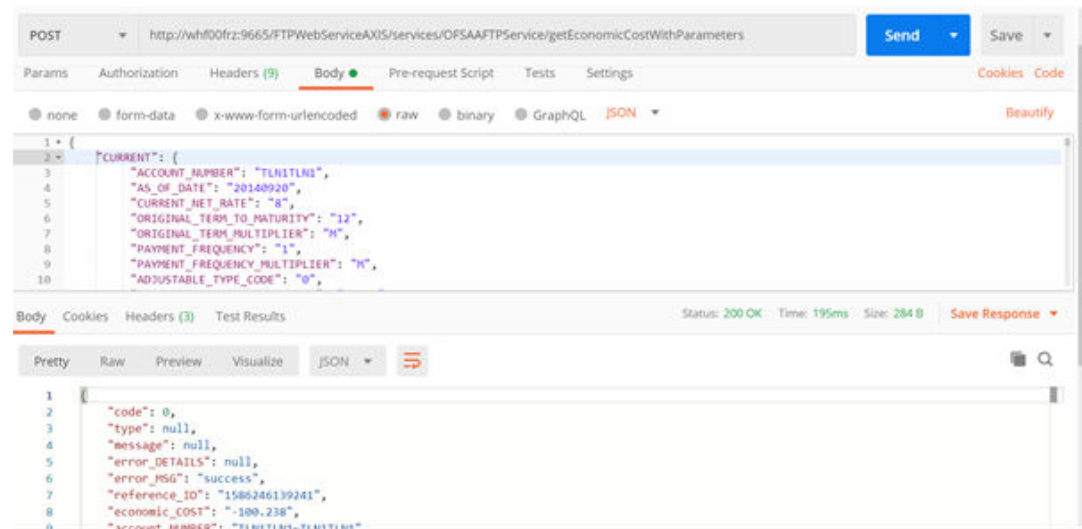
Figure L-3 Web API Testing Tool (example Postman)
