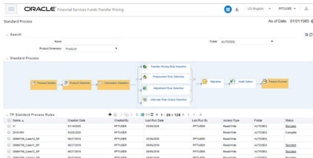
Figure 31-2 FTP Processing - Standard Mode summary page
