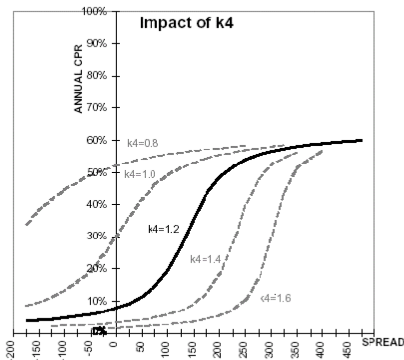
Figure 11-19 Impact of K4 on the Prepayment Curve
