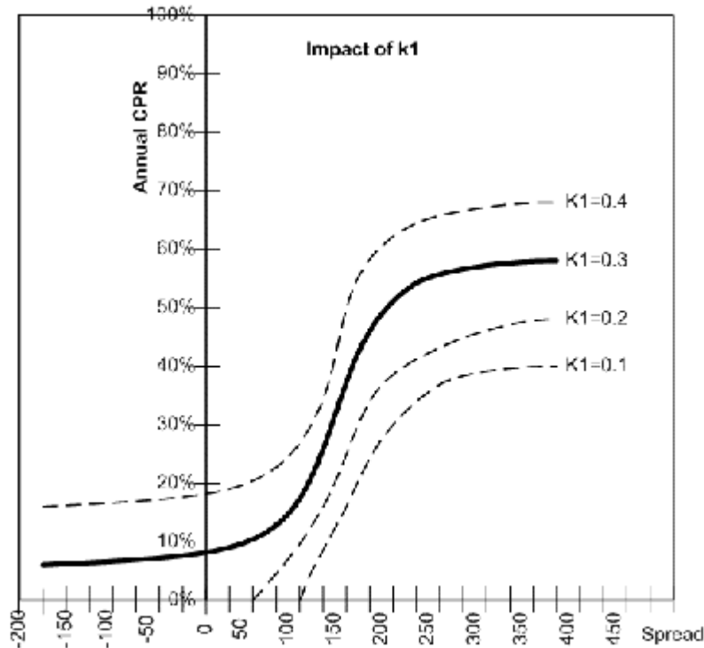
Figure 11-16 Impact of K1 on the Prepayment Curve
