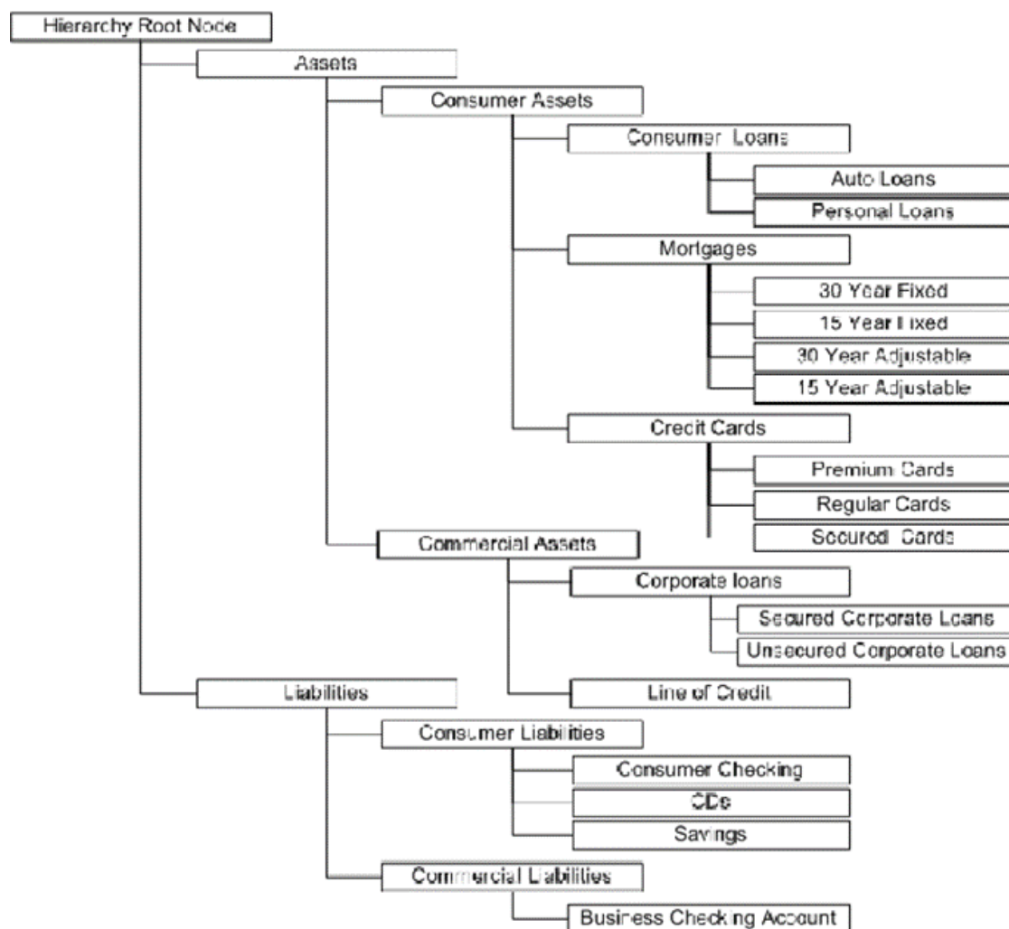
Figure 11-9 Sample Product Hierarchy
