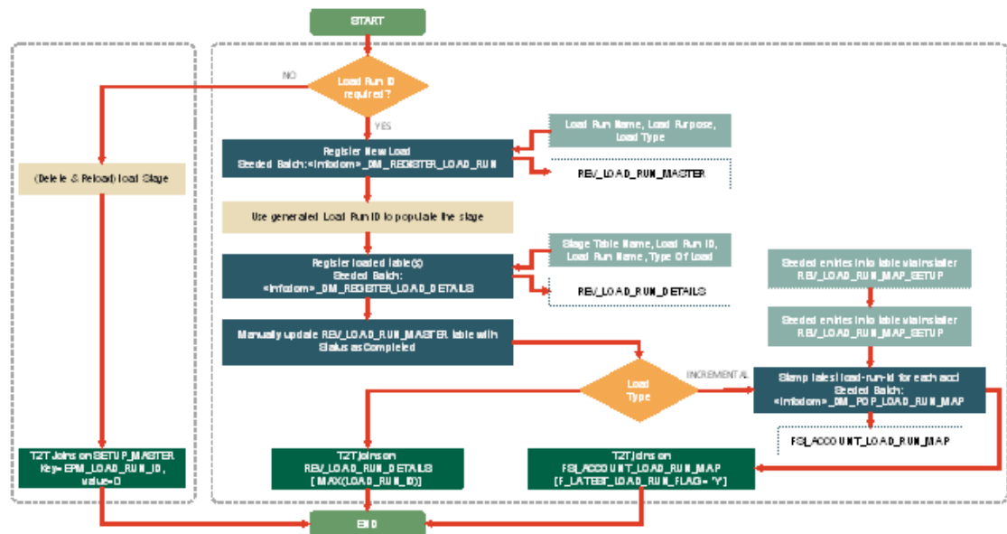
Figure J-1 Load Run ID for T2T Process Flow
