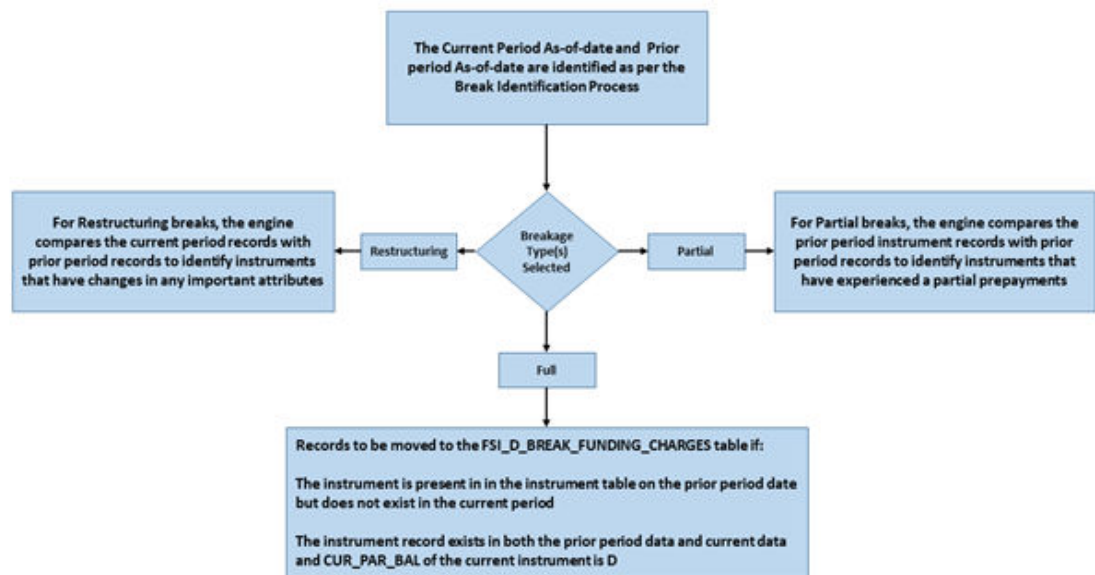
Figure 11-34 Overview of Break Identification Process
