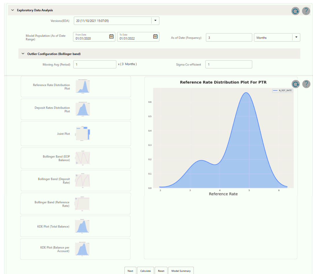
Figure 26-3 Exploratory Data Analysis section
