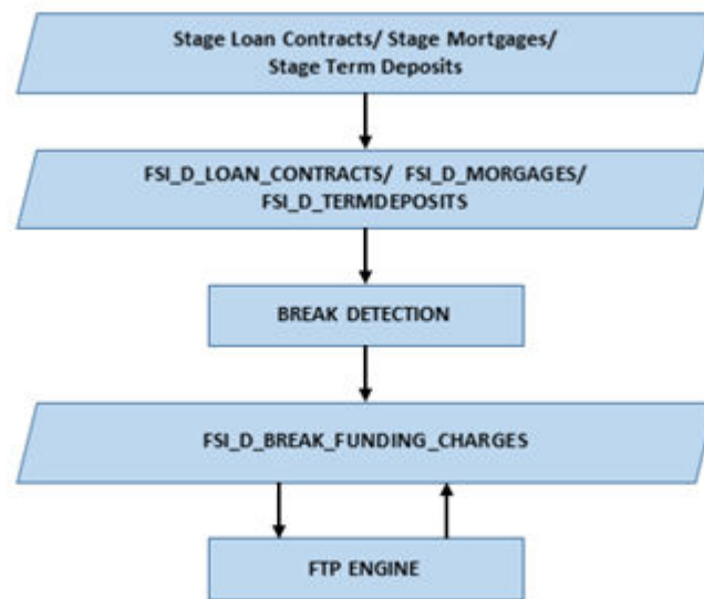
Figure 11-33 Break Identification Process Flow
