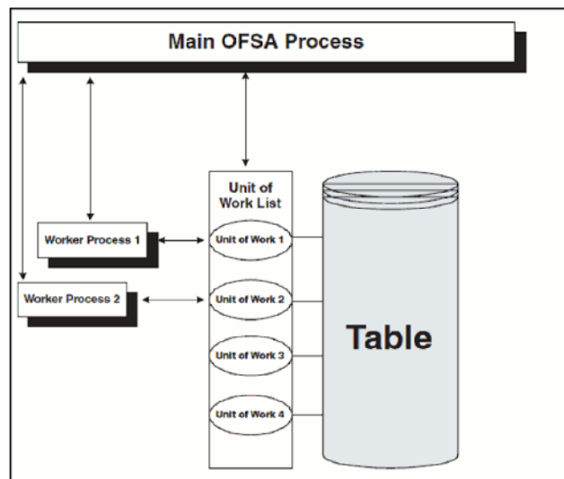
Figure G-11 Basic Multiprocessing principles
