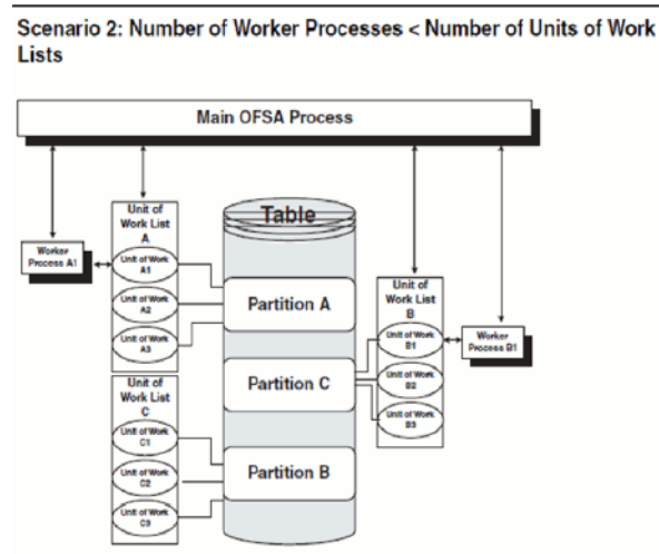
Figure G-13 How different units of work are processed at the same time by different worker processes
