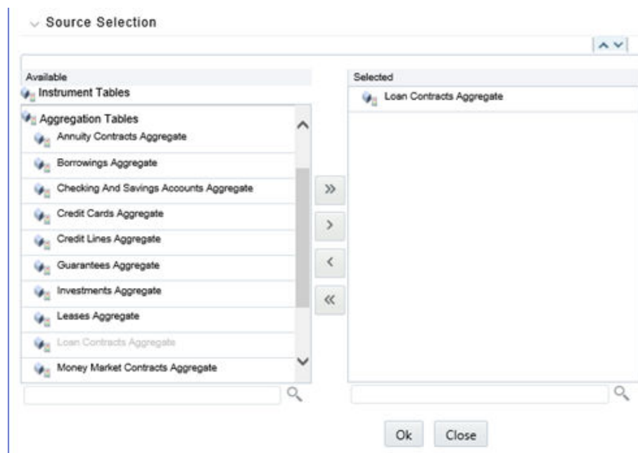
Figure 33-1 Source Selection
