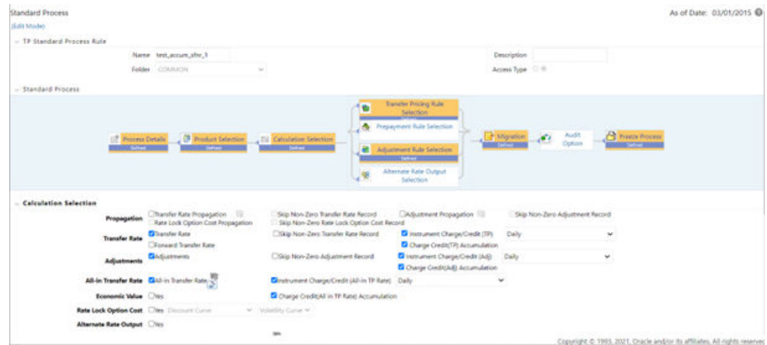
Figure 30-3 Transfer Pricing Rule - Calculation Selection
