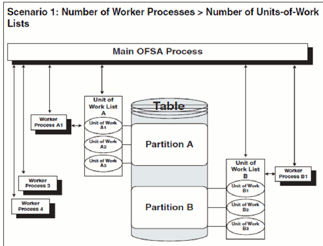
Figure G-12 How the worker processes service multiple unit-of-work lists
