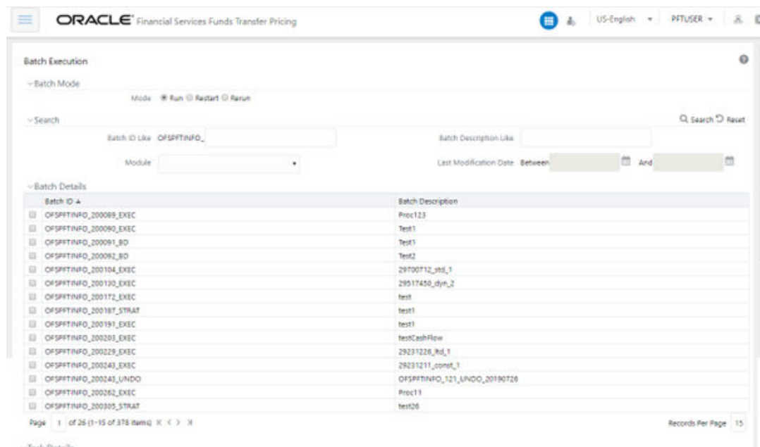
Figure 37-3 Batch Execution
