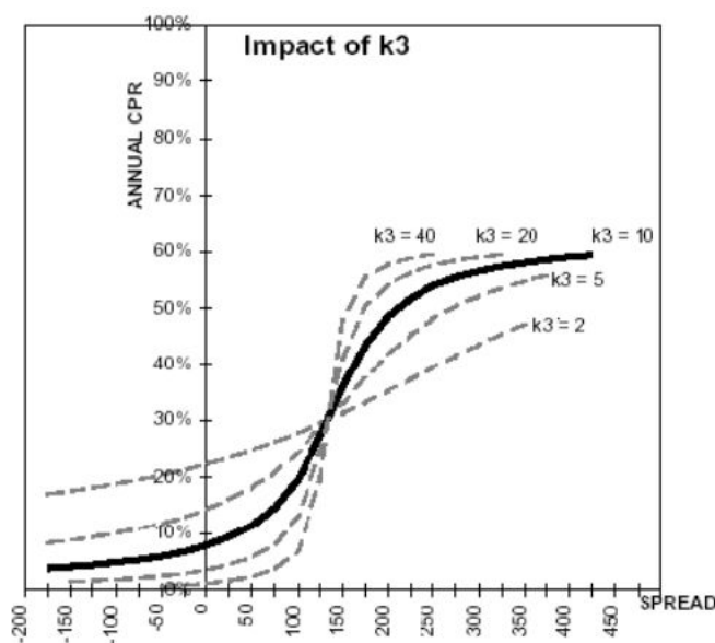
Figure 11-18 Impact of K3 on the Prepayment Curve
