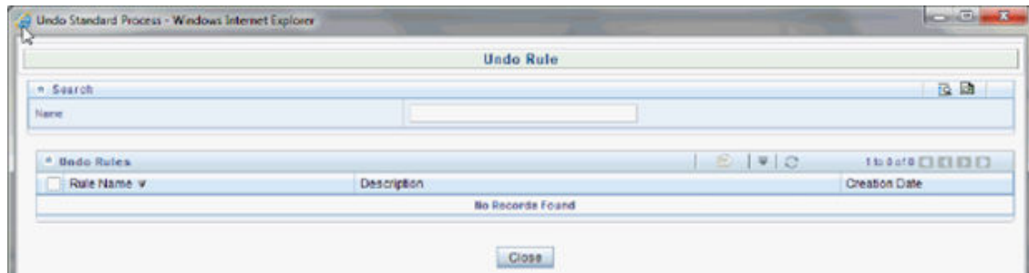
Figure 31-20 Undo Rules
