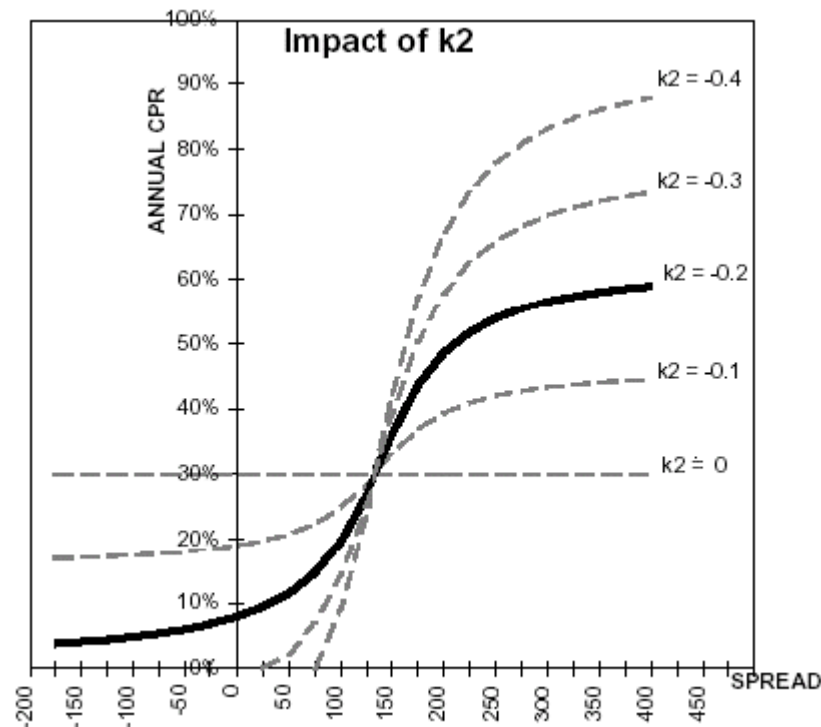
Figure 11-17 Impact of K2 on the Prepayment Curve
