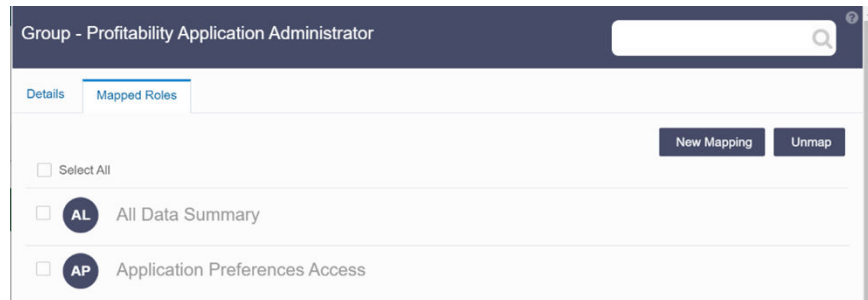
Figure 4-6 Mapped Roles
