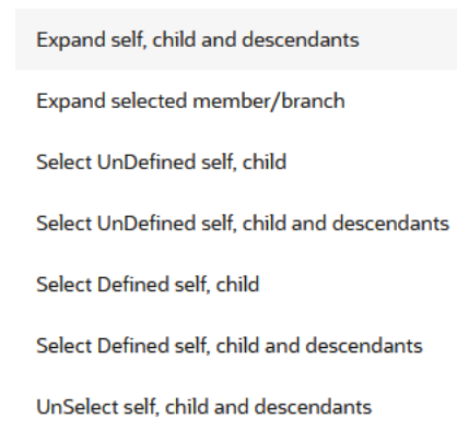
Figure 4-95 Member Tree
