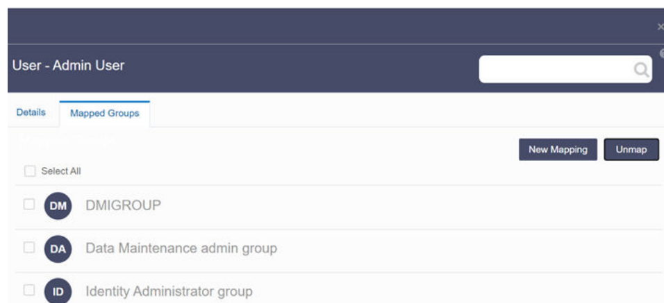
Figure 3-3 Mapped Groups
