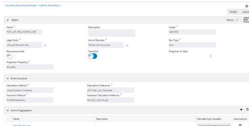
Figure 4-27 The Liability Calculation Window
