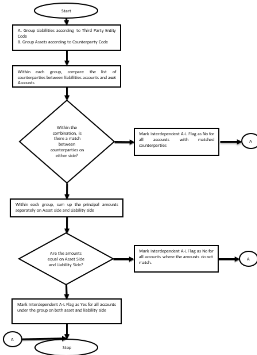
Figure 5-2 Process Flow for the Pair Identification
