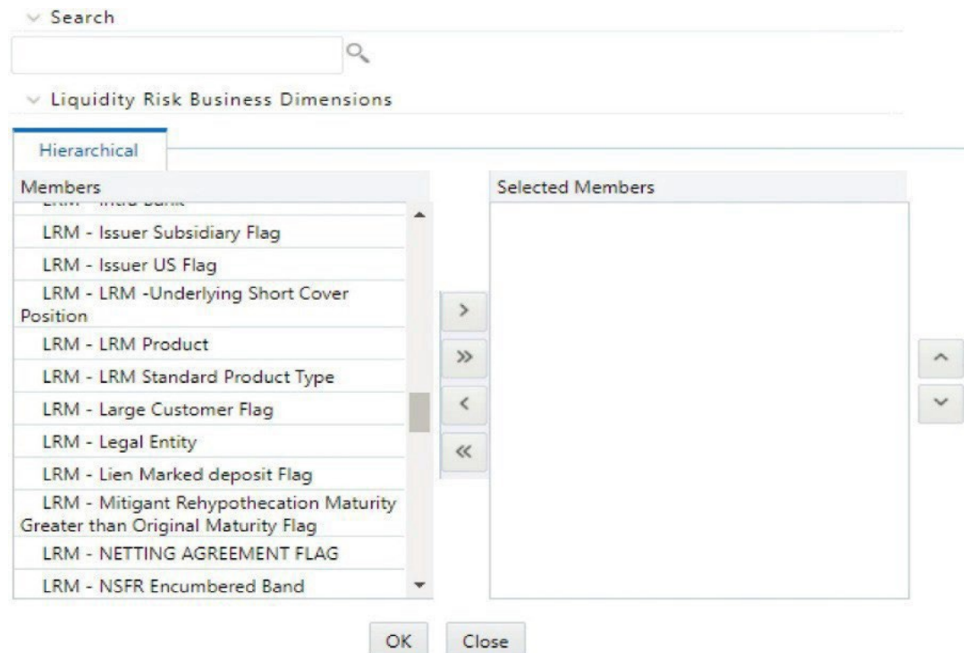
Figure 4-4 Dimension Selection
