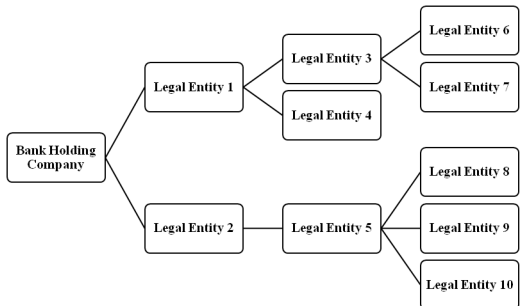
Figure 14-33 Organization Structure
