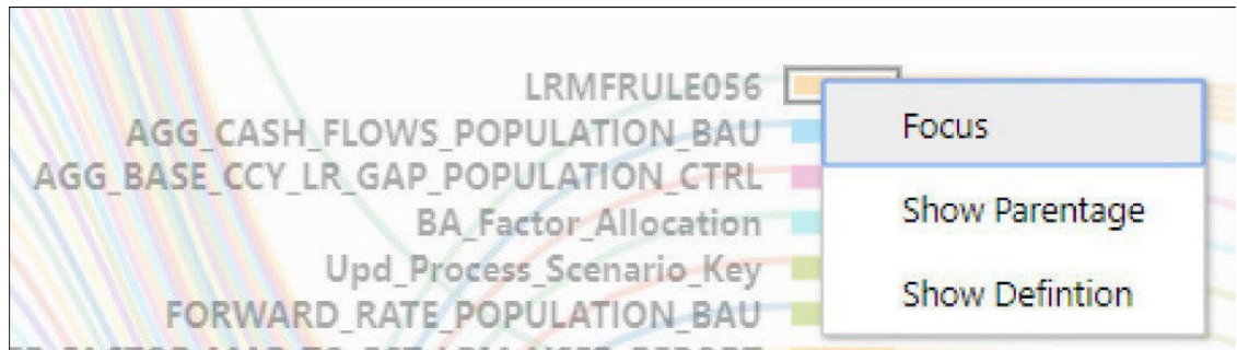
Figure 10-3 Process Details
