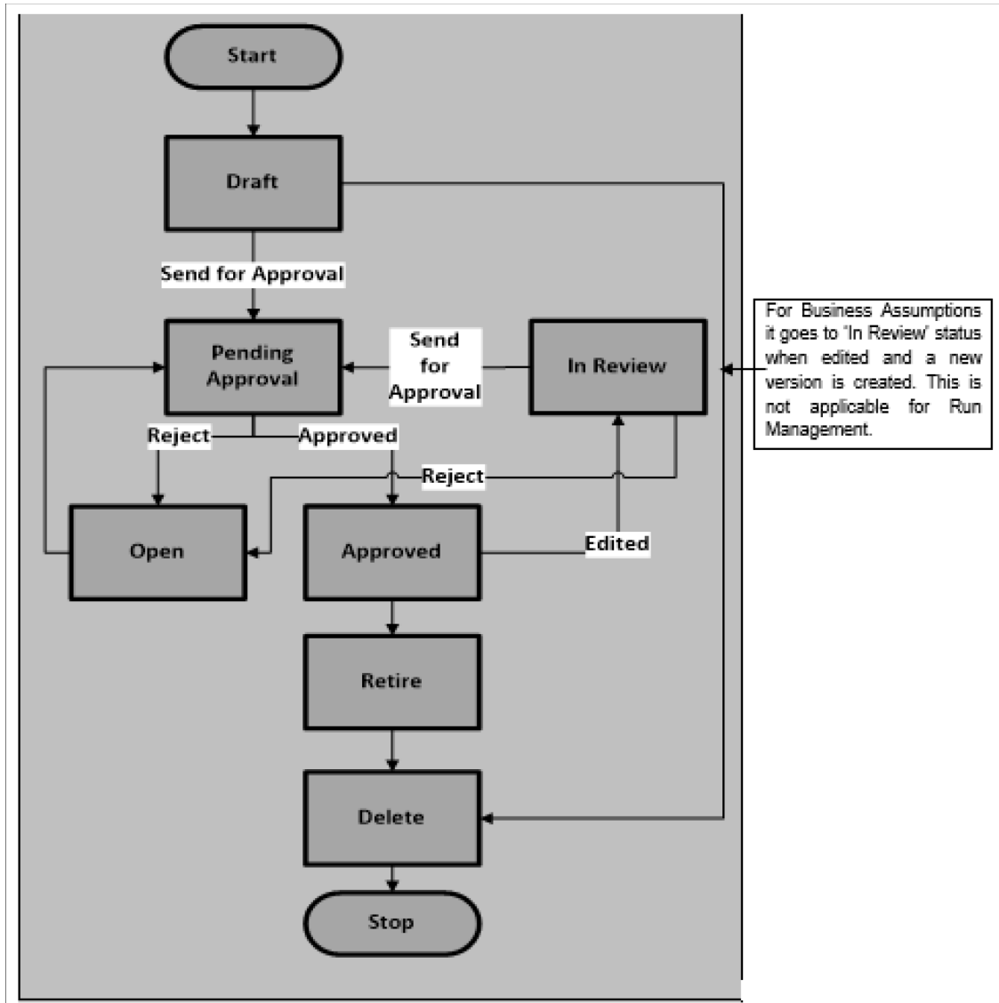
Figure 18-2 Approval Workflow
