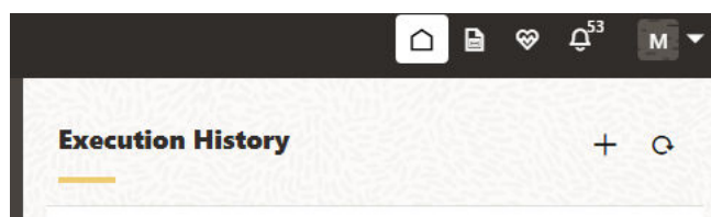
Figure 7-23 Plus icon
