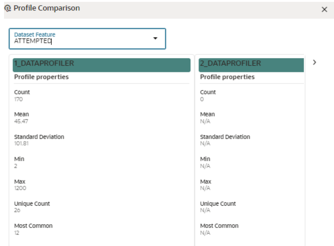
Figure 10-21 Profile Comparison screen
