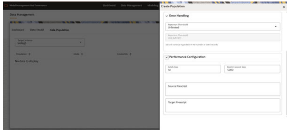
Figure 9-25 Performance Configuration
