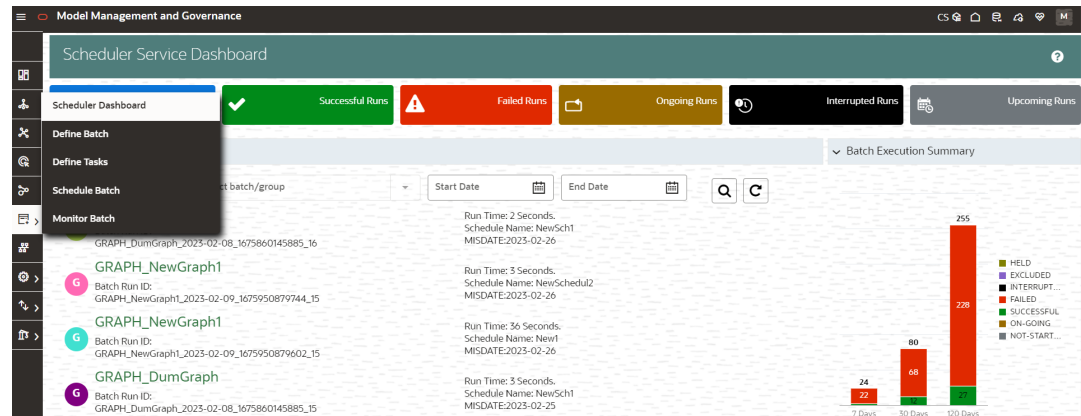
Figure 11-2 Header Details
