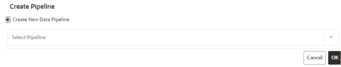
Figure 10-105 Create Pipeline
