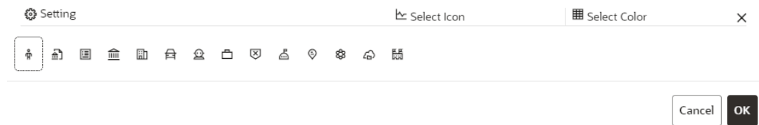
Figure 10-100 Setting
