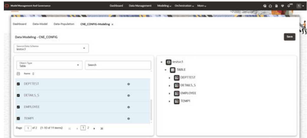
Figure 9-10 Save button
