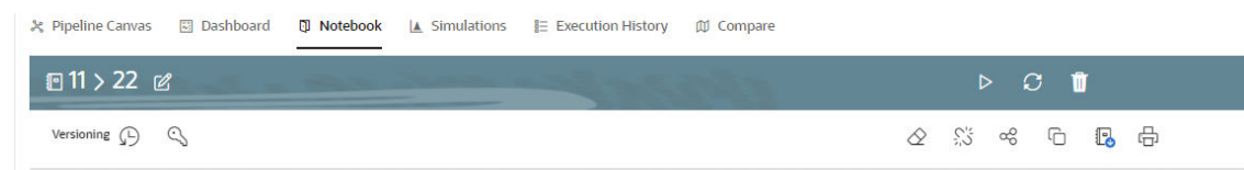
Figure 10-79 Notebook page
