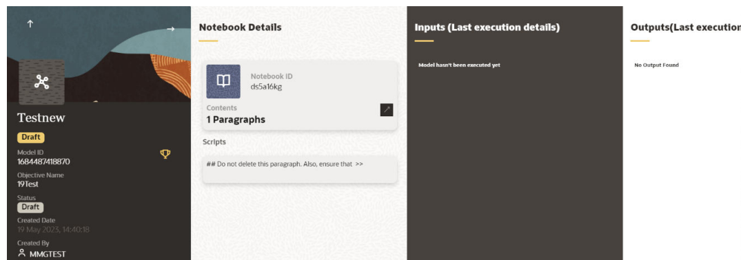
Figure 10-86 Scope Details
