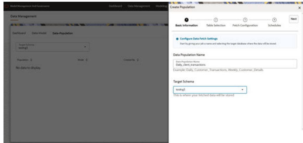
Figure 9-21 Basic Information
