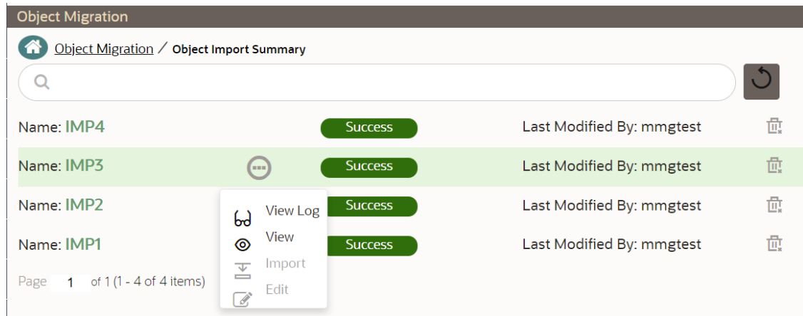
Figure 12-5 Object Migration
