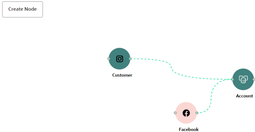
Figure 10-121 Graph page
