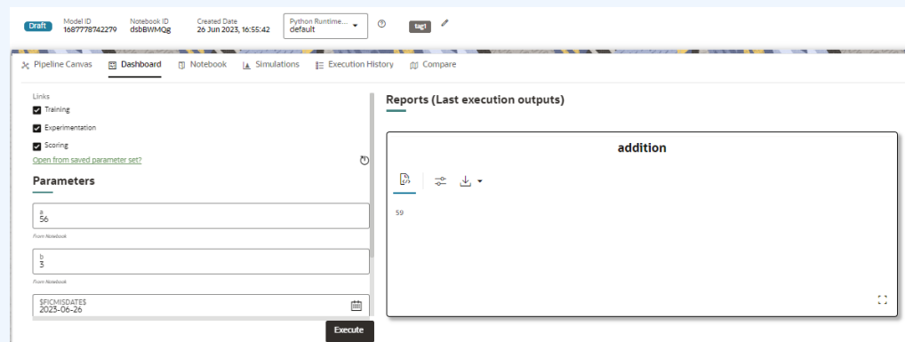
Figure 10-78 Dashboard
