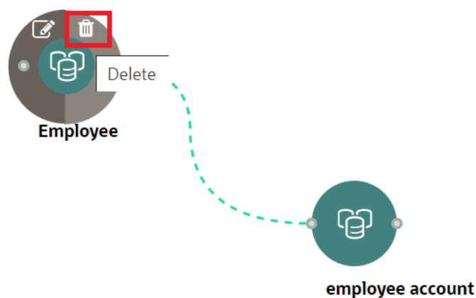
Figure 10-124 Delete Node
