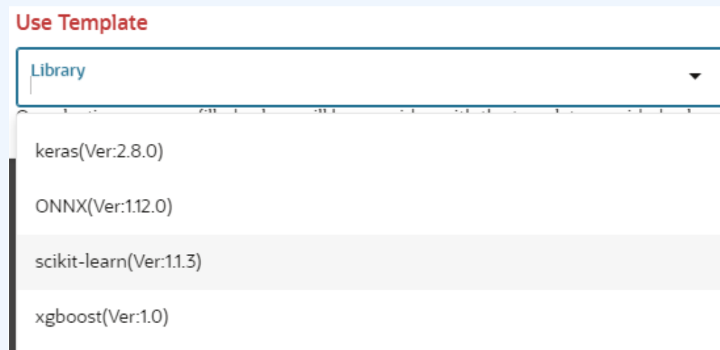
Figure 10-35 Use Template
