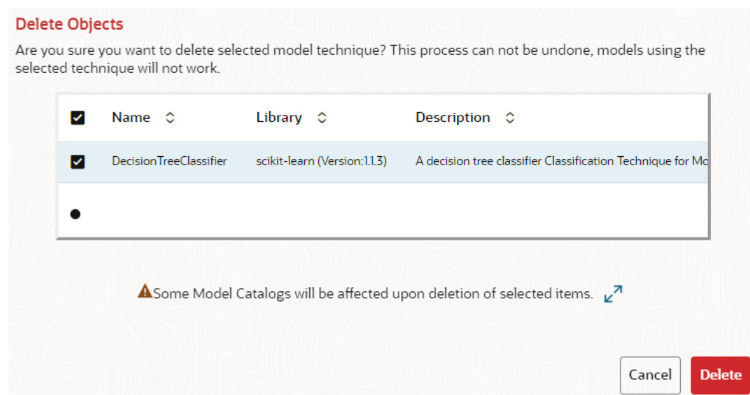
Figure 10-41 Confirmation Message
