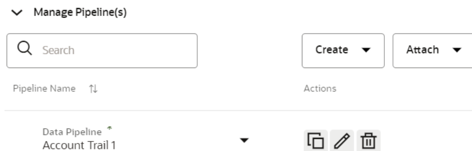
Figure 10-120 Create Pipeline
