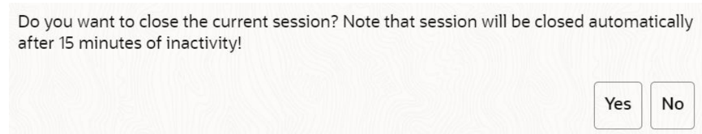
Figure 10-71 Confirmation message
