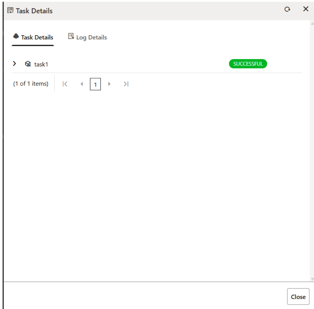
Figure 7-22 Task details
