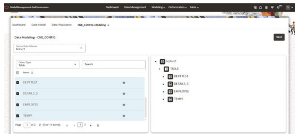
Figure 9-9 Source Schema Name
