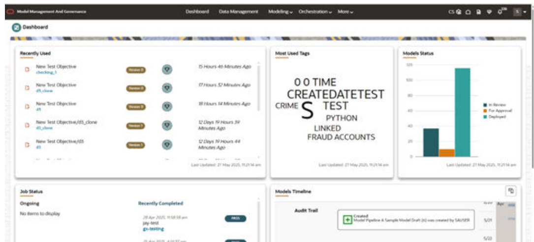
Figure 9-18 Data Population Dashboard
