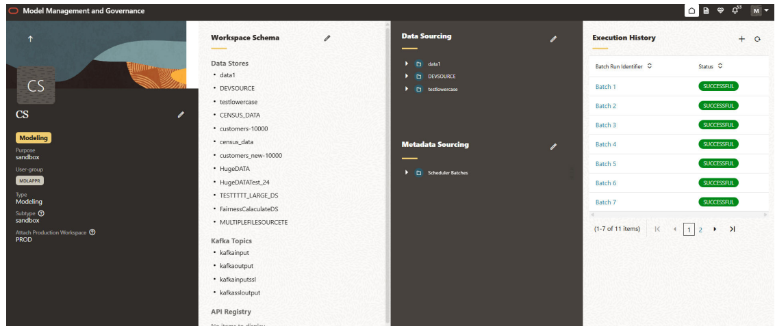
Figure 7-14 Details screen
