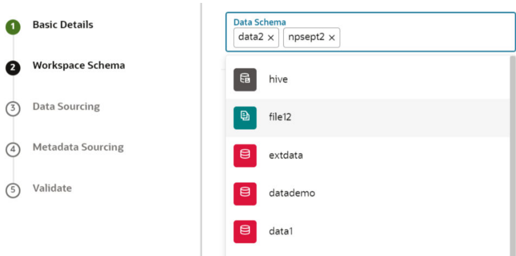
Figure 7-4 Data Schema
