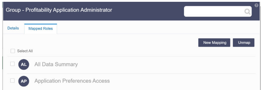
Figure 4-6 Mapped Roles
