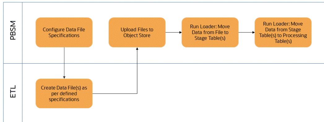
Figure 2-1 Loading External Data into PBSM Cloud Services
