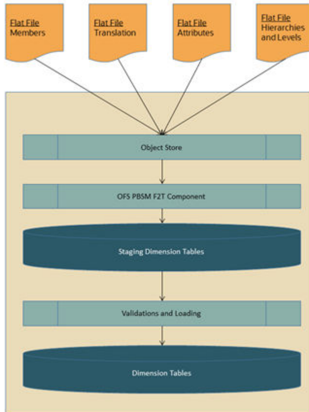
Figure 3-1 Dimension Loading Process
