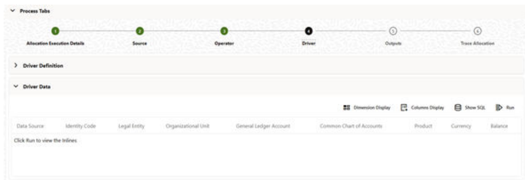
Figure 2-11 Driver Tab
