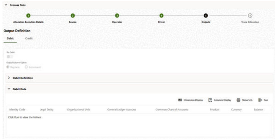
Figure 2-12 Output Tab
