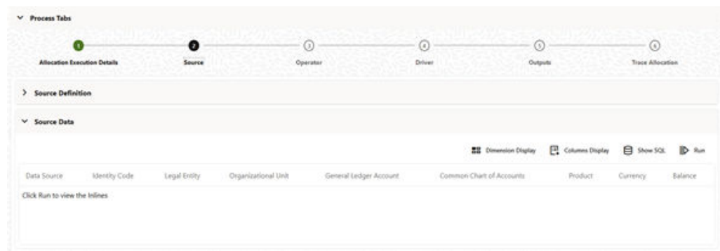
Figure 2-8 Source Tab
