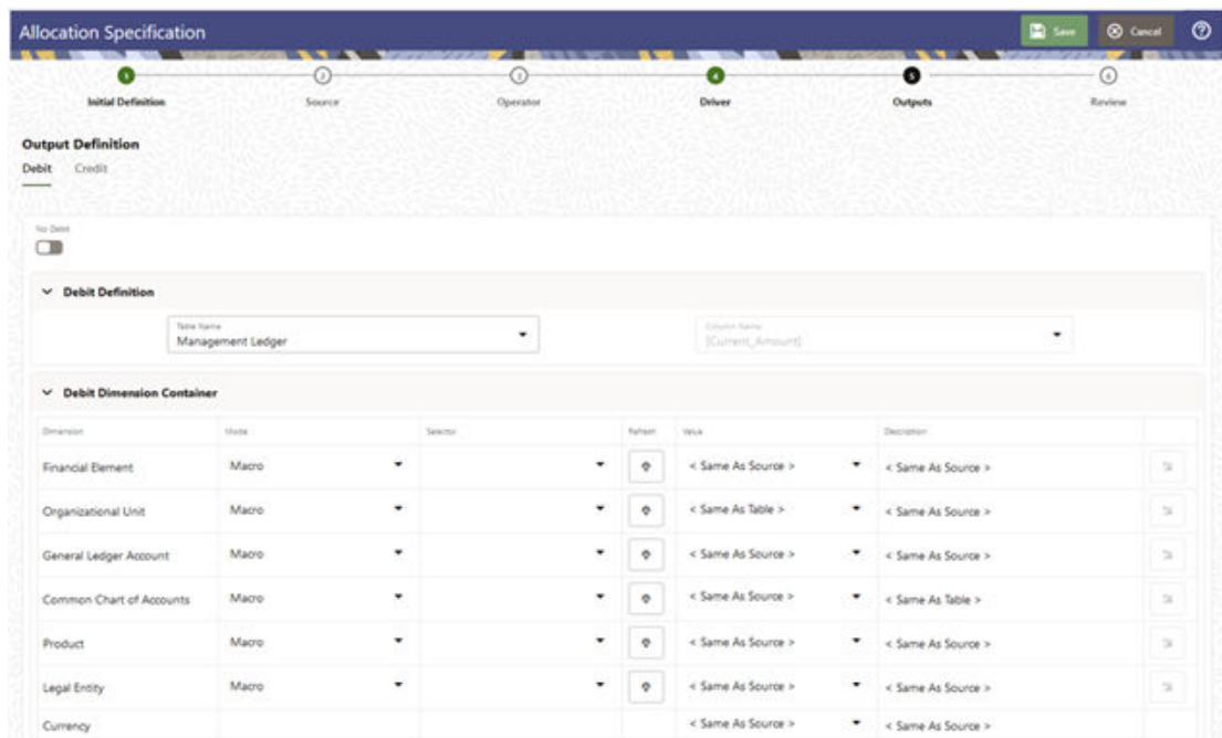
Figure 2-11 Allocation Specification Edit screen - Outputs tab
