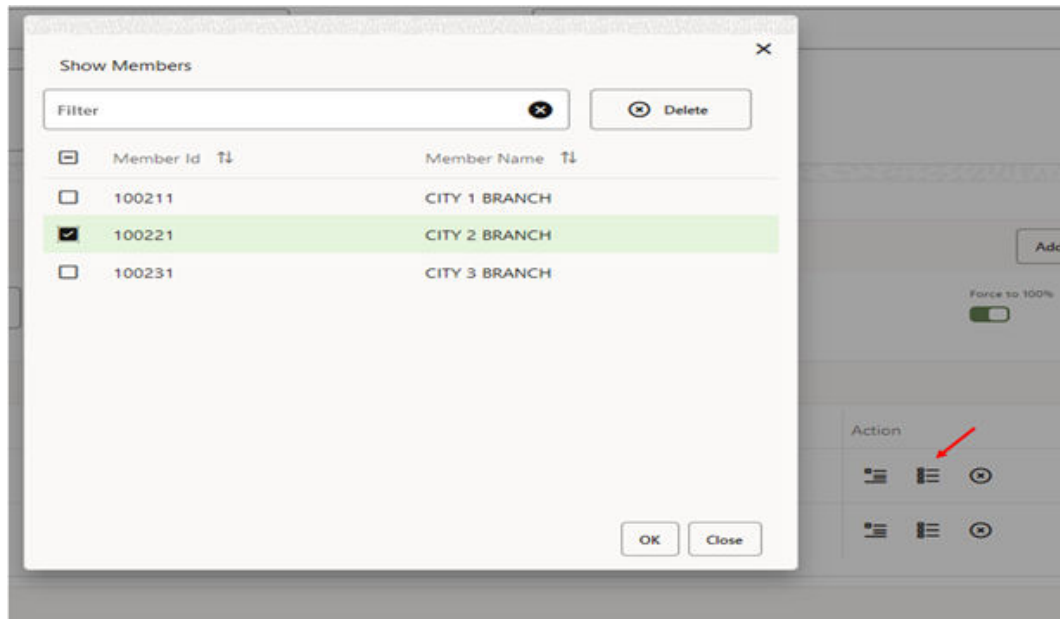
Figure 2-6 Members Browser
