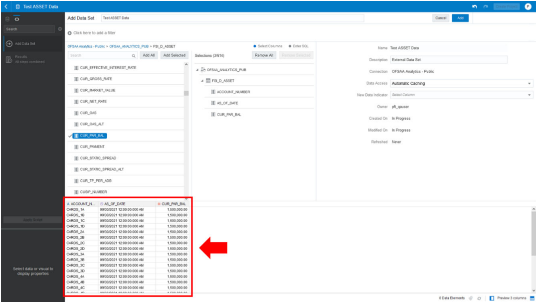
Figure 8-8 Data Results
