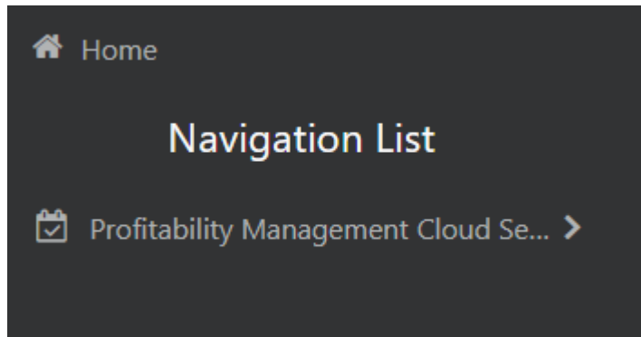
Figure 2-6 Navigation Path
