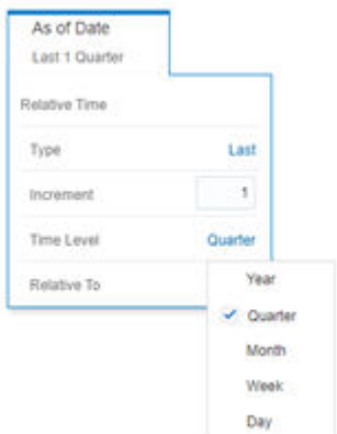
Figure 8-153 As-of-Date Selection
