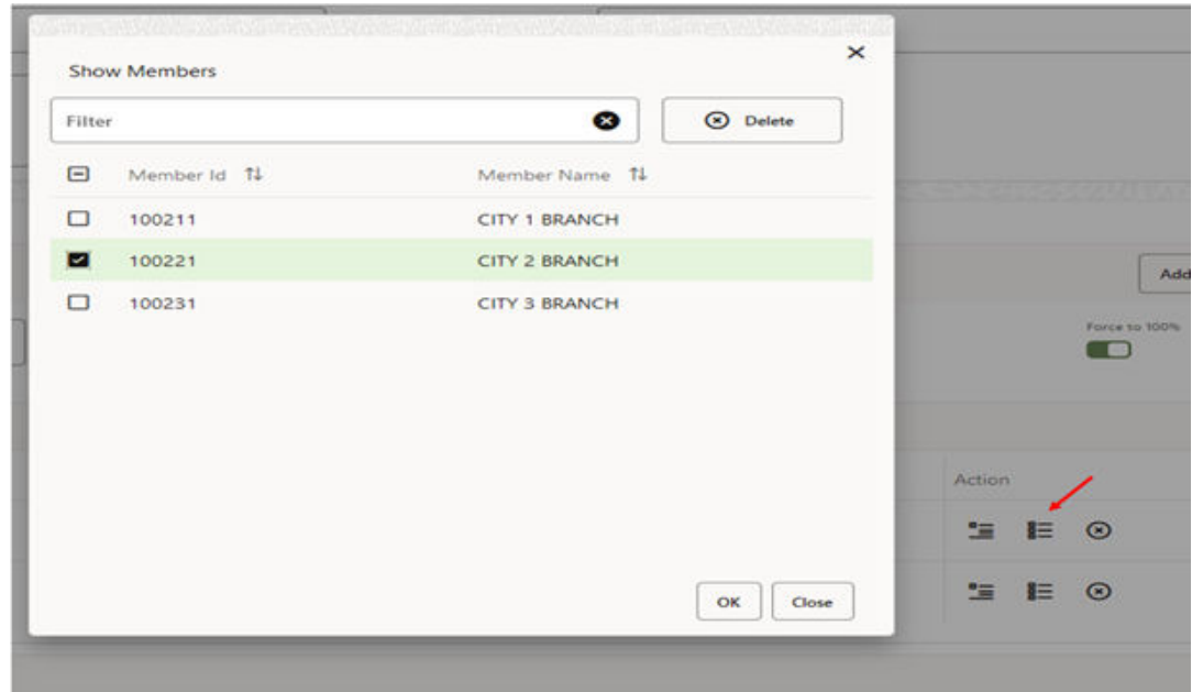
Figure 6-74 Members Browser
