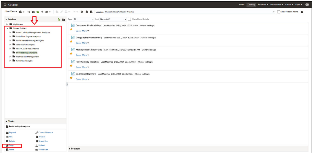
Figure 8-14 Folders
