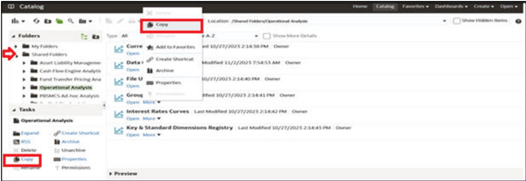
Figure 8-13 Copy Option
