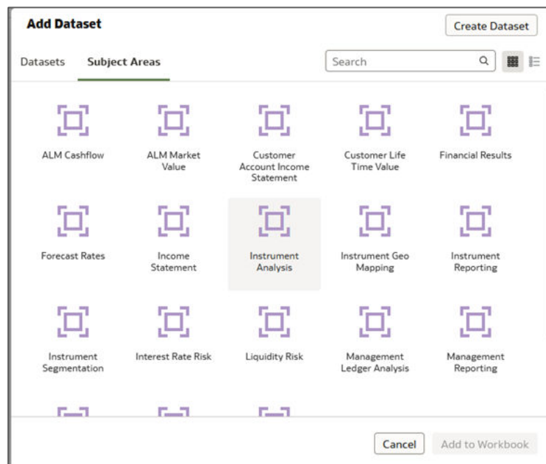
Figure 8-18 Subject Areas
