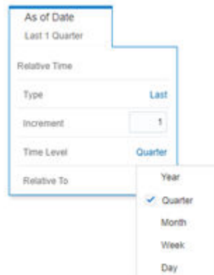
Figure 8-137 As-of-Date Selection
