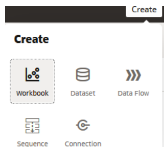
Figure 8-17 Create
