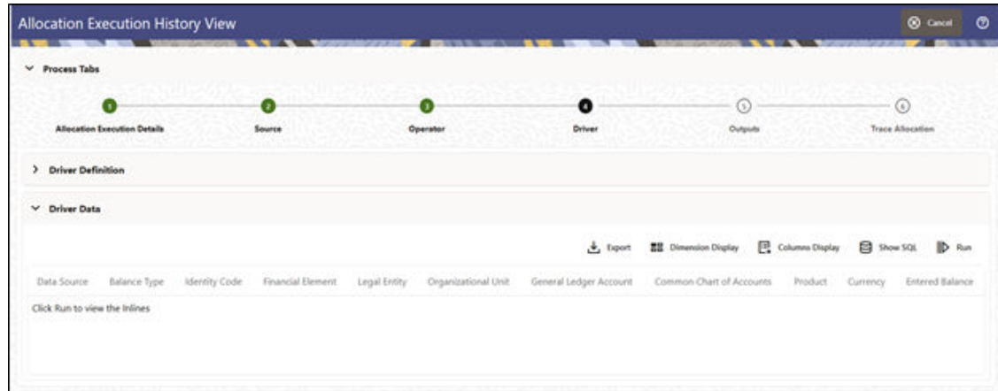
Figure 6-65 Driver Tab
