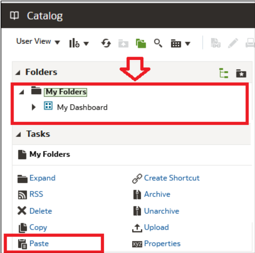
Figure 8-15 My Folders
