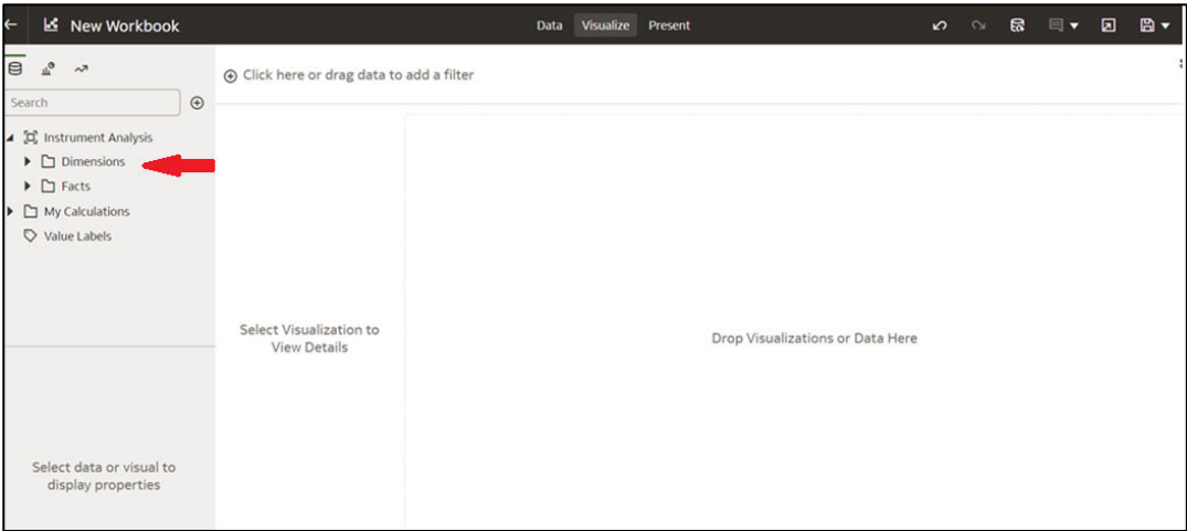
Figure 8-19 New Workbook
