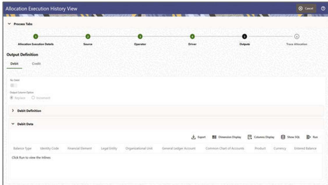
Figure 6-66 Output Tab
