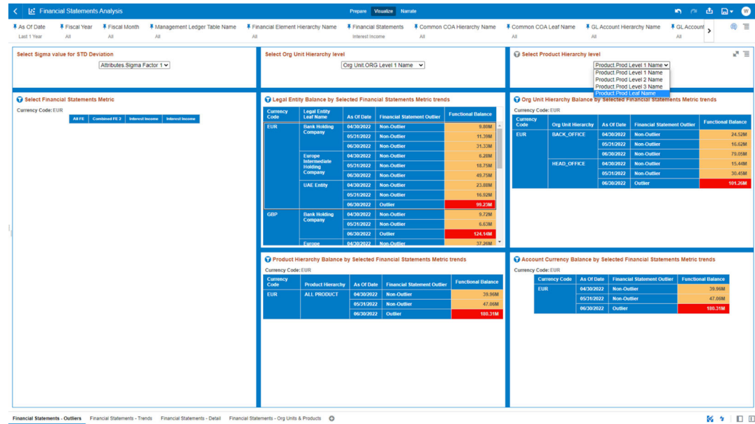
Figure 8-170 Outliers Selection
