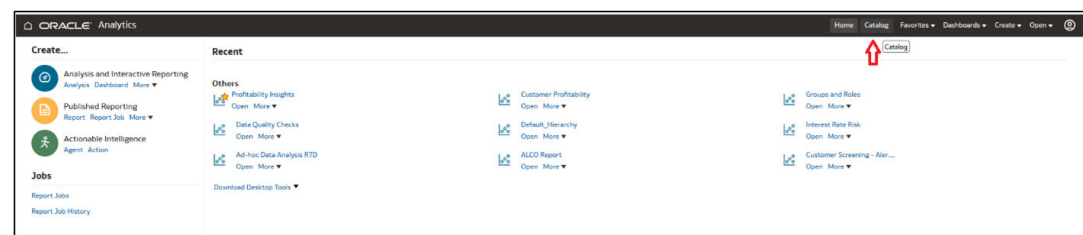
Figure 8-12 Catalog
