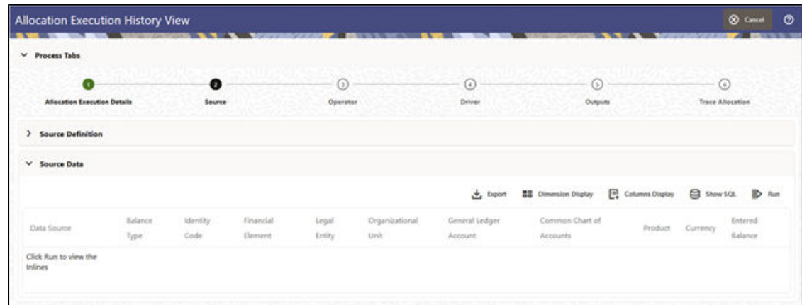
Figure 6-62 Source Tab
